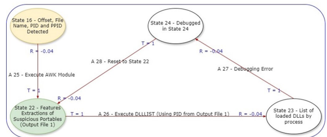
Fig. 7: AWK Module Features Extractions
