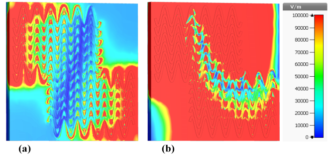
Fig. 10. Distributions of the electric field across the proposed metamaterial structure: (a) E-field at 0.437 THz, and (b) E-field at 0.75 THz.
