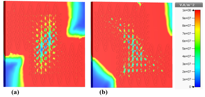
Fig. 13. Power flow over the proposed metamaterial structure: (a) at 0.437 THz, and (b) at 0.75 THz.
