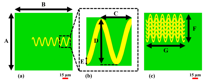
Fig. 1. Proposed metamaterial model#1 of a perfect absorber showing a single wave; (a) one wave, (b) one \lambda , and (c) model#2.
