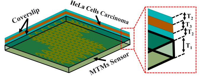
Fig. 17. A layer of biological tissue (either healthy cervical tissue or cancerous cervical tissue) is placed on top of the proposed metamaterial biosensor.
