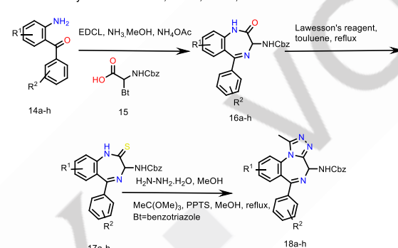
Scheme 3: Synthesis of 14a-h, 16a-h, 17a-h, and 18a-h.
