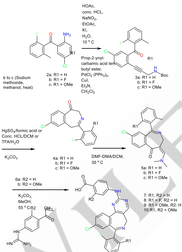
Figure 14. Synthesis of compound 7 to compound 10. [49]
