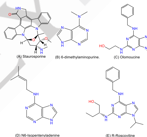
Figure 11. The development of R-Roscovitine/Seliciclib.
