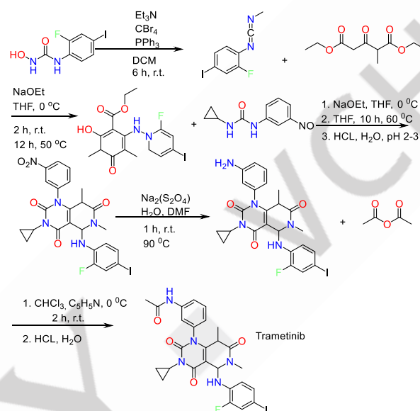
Figure 26. Synthesis of Trametinib [60]
