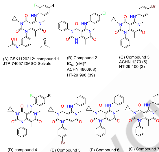
Figure 25. The development of Trametinib. [59]
