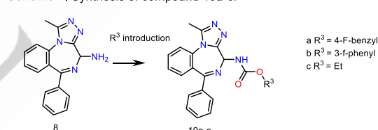
Scheme 5: Chiral Separation of Compound 19c
