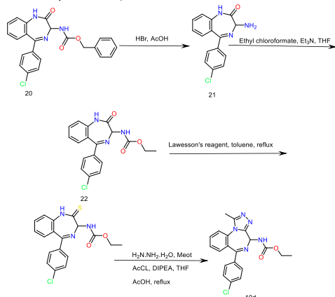
Scheme 6. Synthesis of compound 19d
