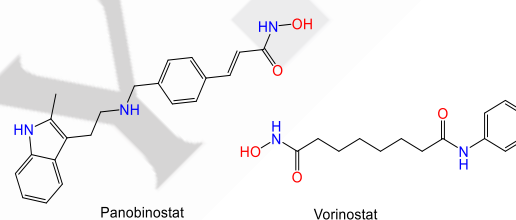
Figure 31. Structure of Panobinostat and Vorinostat. [78]
