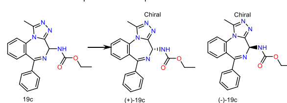
Scheme 5: Chiral Separation of Compound 19c
