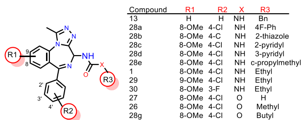
Figure 24. SAR around the BZD Acetamide Template.
