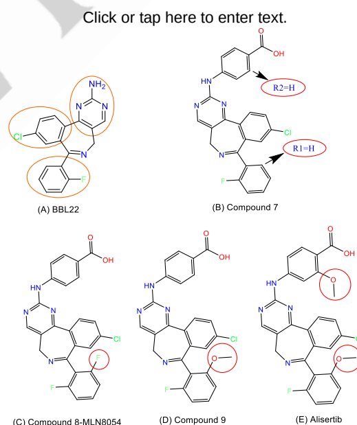
Figure 13. The development of Alisertib.
