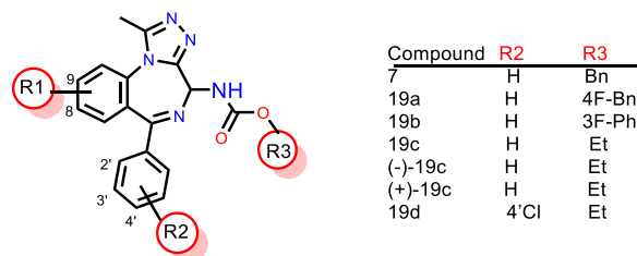
Figure 23. Substitution of R2 and R3 for optimisation.
