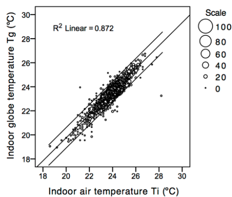
Figure 5. Correlation between indoor air and globe temperatures. Outer lines indicate 95% CI of the regression line.
