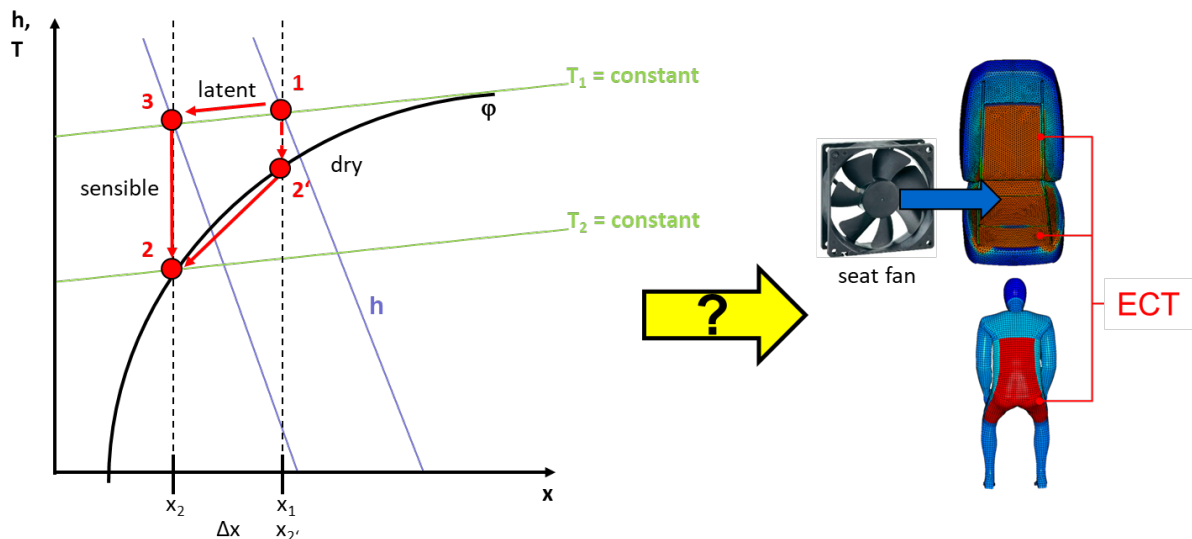
Figure 2. General idea for the calculation of ECT; left-hand side: generalized Mollier diagram, right-hand side: cooling of the contact area between the human body and the seat surface for a ventilated seat; T_1, T_2 : isotherms, \phi : relative humidity, h : lines of constant enthalpy, x_1, x_2, x_2' : specific humidity, \Delta x : difference in specific humidity between the different states 1, 2, 2', 3
