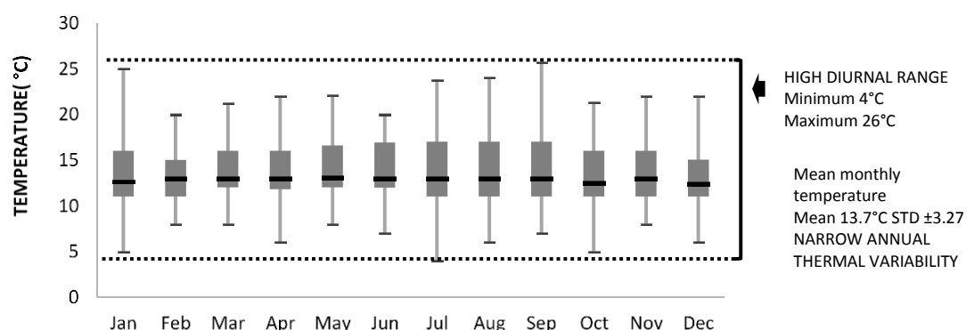
Figure 2: Quito Dry-bulb temperature (°C) – Source: NREL
