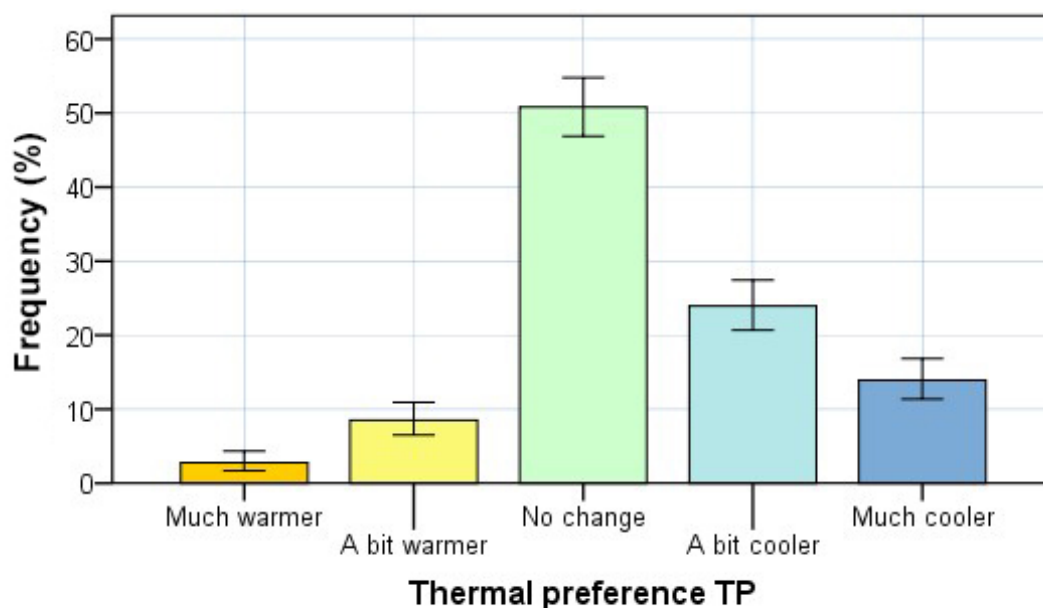
Figure 23. Thermal preference cases frequency graph.
