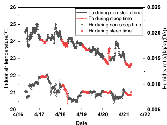
Figure 1. Indoor air temperature and humidity ratio during a typical week
