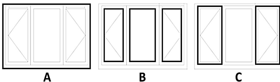
Figure 1. Window and glazed/semi-glazed door details captured in the OAST: total area (A); glazed area (B); and operable area (C)
