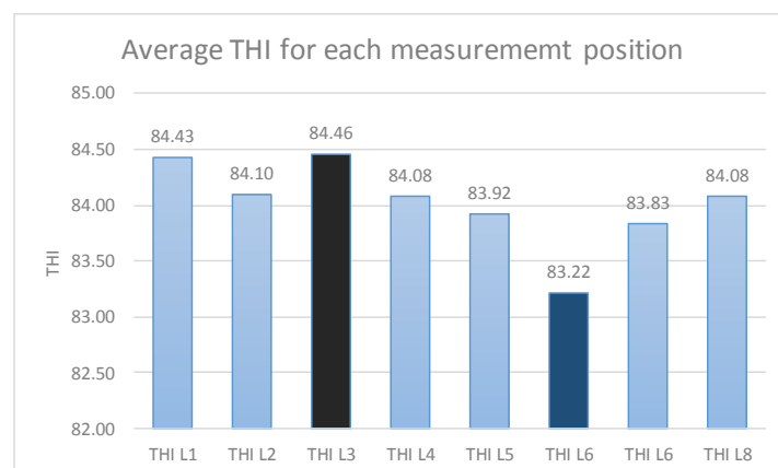
Figure 11. Average THI for each measurement position CFD Results
