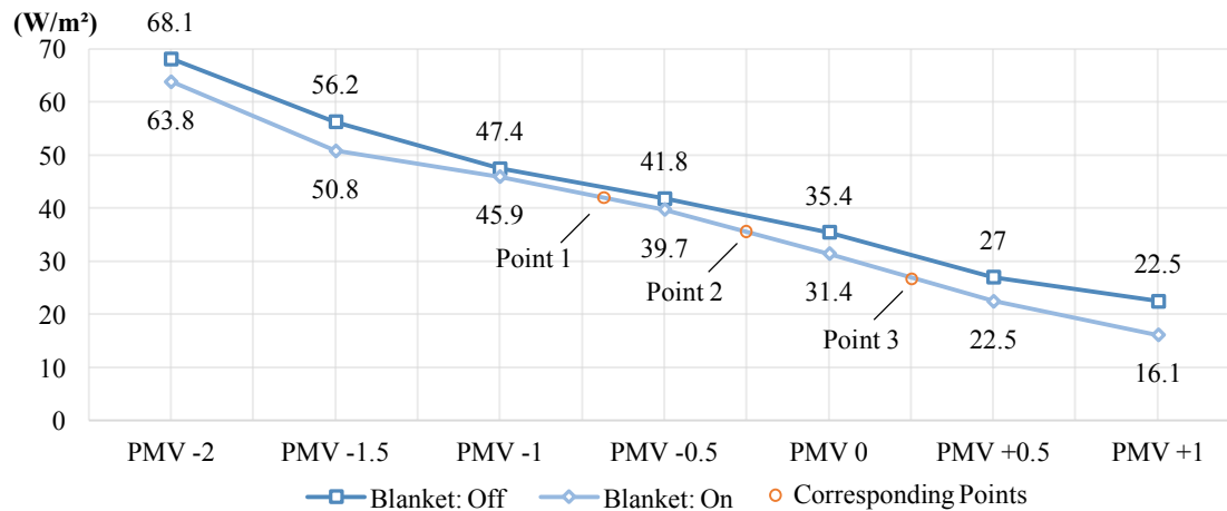
Figure 7 Manikin whole-body heat loss for blanket on or off versus PMV conditions (manikin heat flux uncertainty estimated as \pm 1 Watt).
