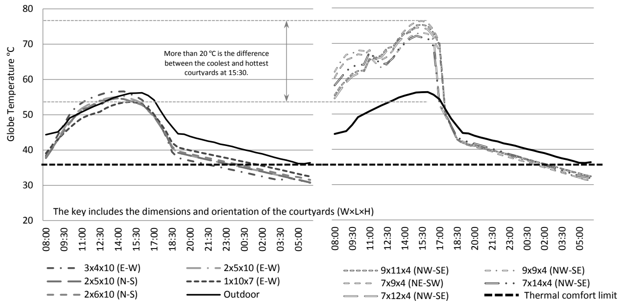
Figure 5. The hourly Globe Temperature in the five most thermally efficient courtyards (left) and the worst five courtyards (right)
