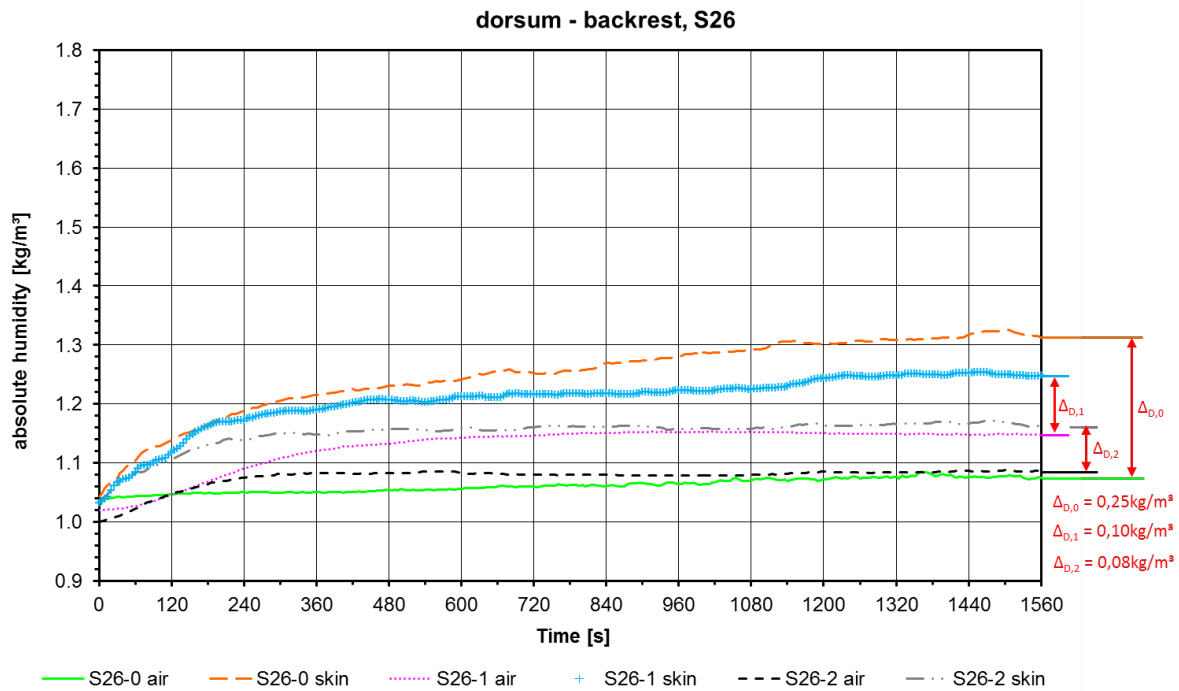
Figure 8: Transient behaviour of the absolute humidity at the contact interface between the dorsum and the backrest of the seat; S26-0 to S26-2: test scenarios for 26 °C and fan levels of 0 %, 35 % and 65 %
