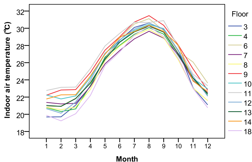
Figure 4 Indoor and outdoor air temperature according to floors.
