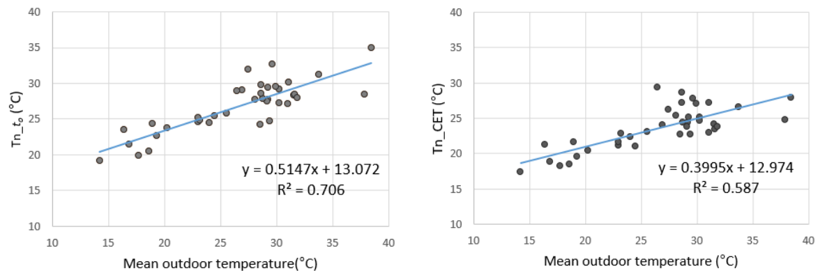
Figure 5. MSTC-NVB model for t_o and CET.
