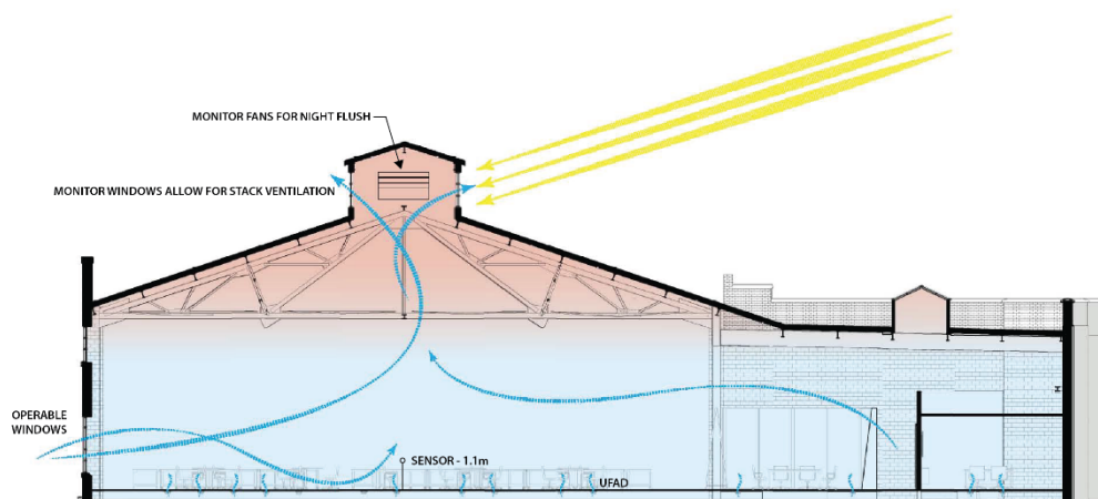
Figure 1. An east-west building section showing airflow under natural ventilation. The building's tall open office allows for stratified air to accumulate at the top of the space and easily exhausted via operable monitor windows.
