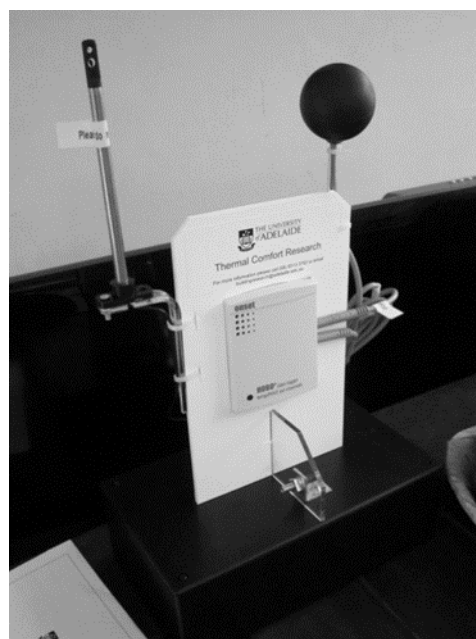
Figure 3. Monitoring device used in 2013/14 study
