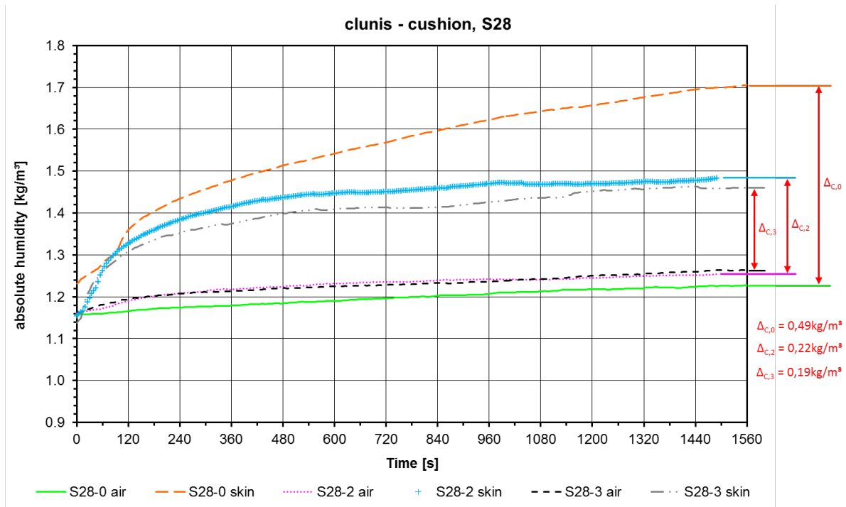
Figure 11: Transient behaviour of the absolute humidity at the contact interface between the clunis and the cushion of the seat; S28-0 to S28-3: test scenarios for 28 °C and fan levels of 0 %, 65 % and 100 %
