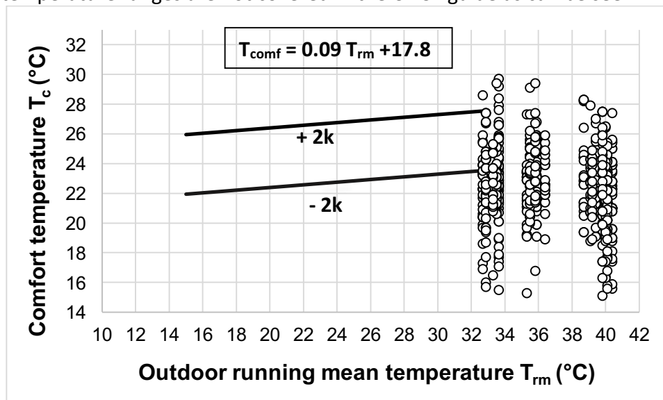
Figure 30. Relationship of the Griffiths' indoor comfort temperature with the running mean outdoor temperature super-imposed over the CIBSE standard (Each point represents a single vote.)
