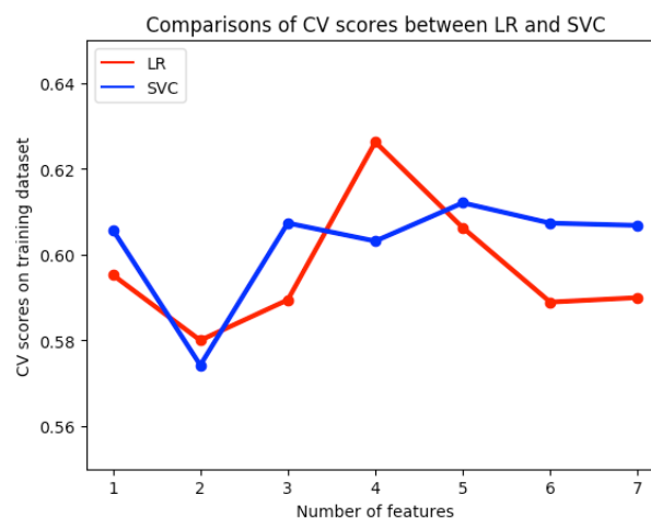
Figure 8. Comparison of CV scores between LR and SVC on various feature subset
