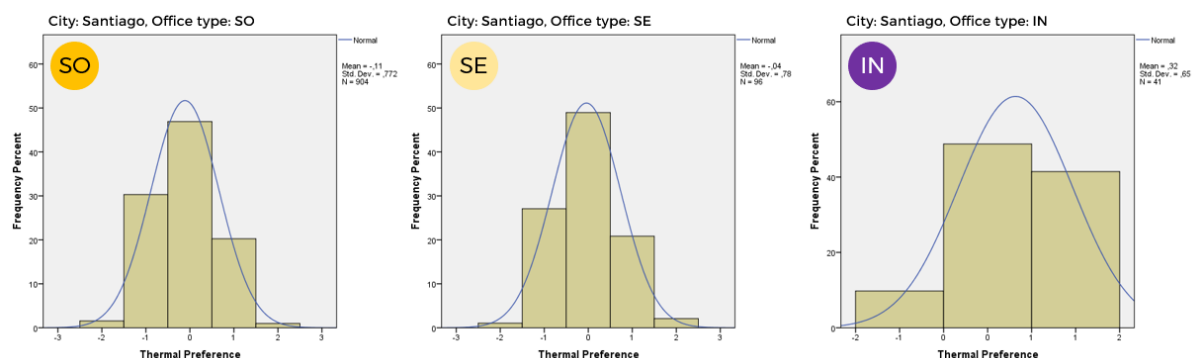
Figure 8. Distribution of subjective thermal preference Santiago
