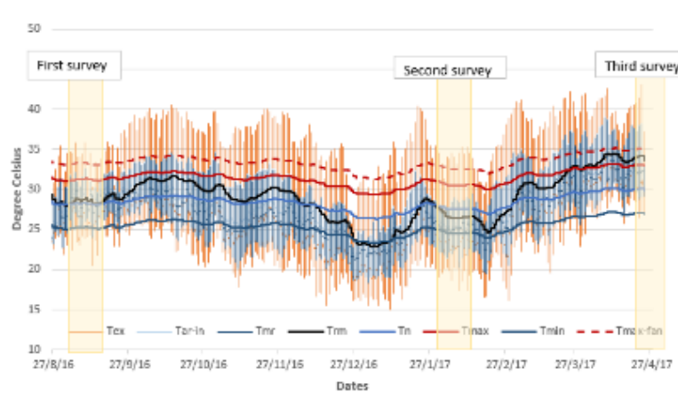
B - FEES temperature time series Figure 6: Temperature time series of the theatres
