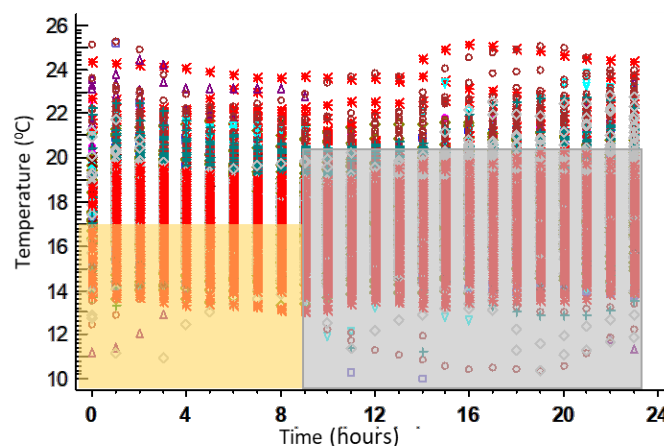
Figure 2: Distribution of daytime temperatures (°C) in the winter months in the group of dwellings compared to Heating setpoint temperatures, in accordance with the Energy Rating procedure and characterisation of CTE-HE demand. Night temperature setpoint (yellow) and day temperature setpoint (grey).
