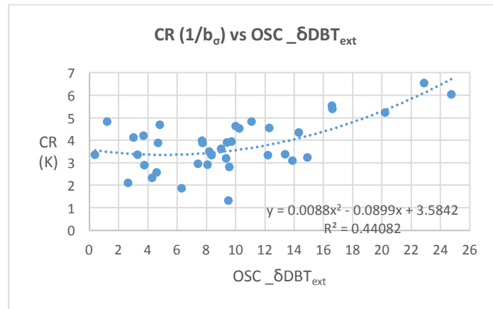
Figure 15. Polynomial dispersion diagram for the comfort range that was obtained from the standard deviation, based on the average temperature of the exterior
