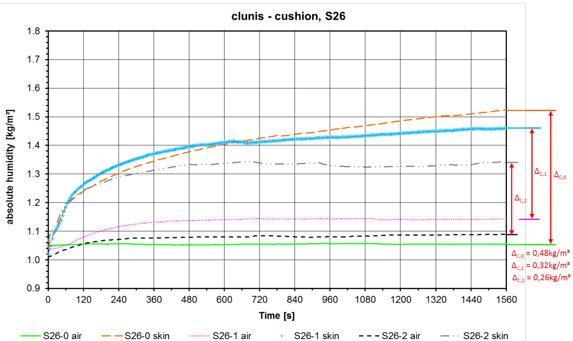
Figure 9: Transient behaviour of the absolute humidity at the contact interface between the clunus and the cushion of the seat; S26-0 to S26-2: test scenarios for 26 °C and fan levels of 0 %, 35 % and 65 %
