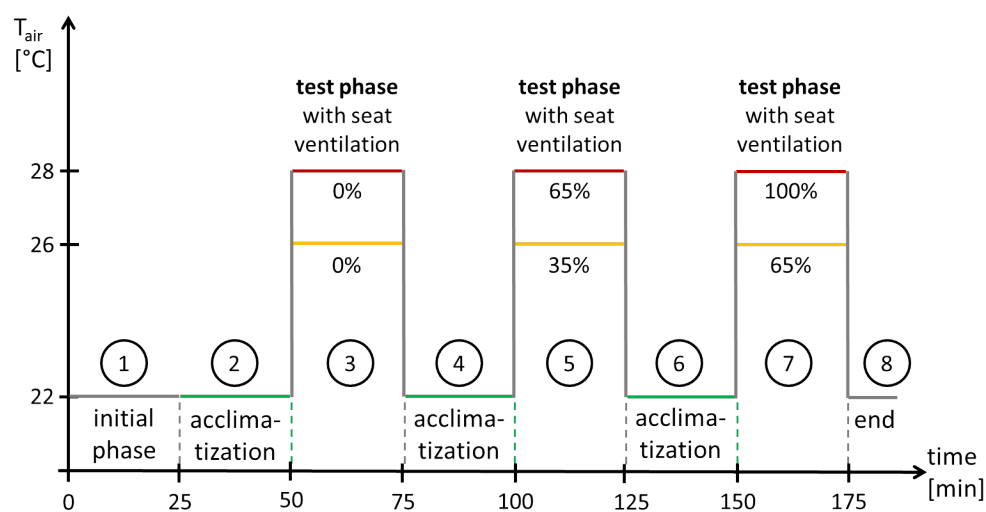
Figure 5: Example of test cycle for a single subject; schematic shows the two tested summer scenarios at temperatures of 26 °C and 28 °C; percentages indicate the relative fan speed, where 0 % means fan is switched off and 100 % represents the highest possible fan speed
