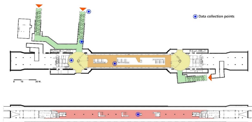
Figure 5 Plan showing location of Thermal comfort meter setup
