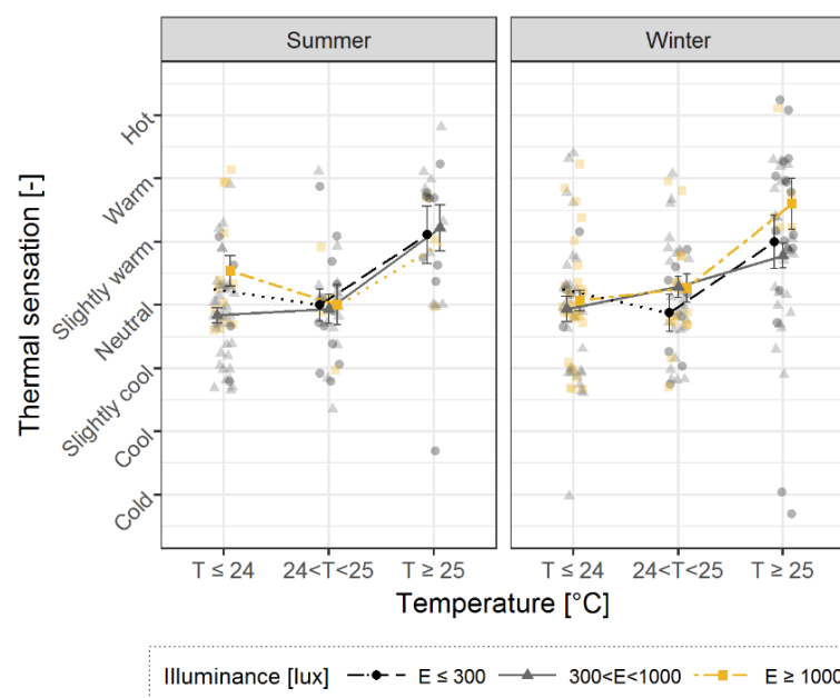
Figure 2. Thermal sensation response means \pm s.e.m. according to the two seasons, temperature and illuminance levels.
