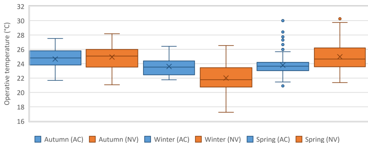
Figure 5. Box plot of operative temperature for AC and NV periods. The line within each box is the median, the cross is the mean, the edges of the box are the 25th and 75th percentiles, the dots are the outliers.
