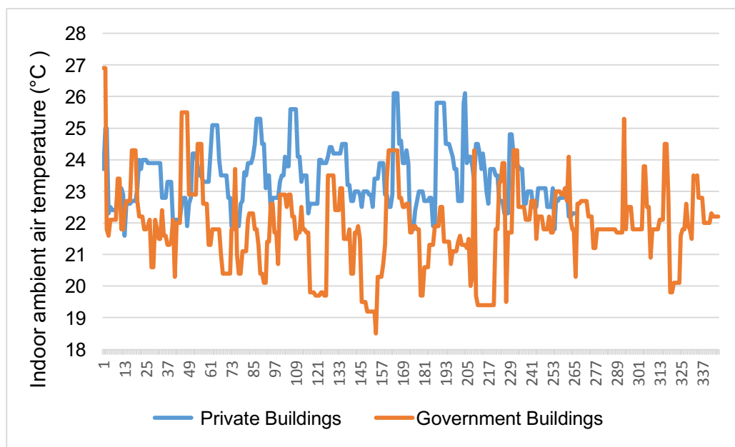
Figure 18. Chart showing indoor air temperatures ( T_a ) in government office buildings vs. private office buildings.
