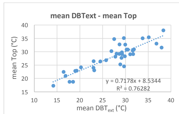
Figure 12. Relationship between mean indoor Top and mean DBText
