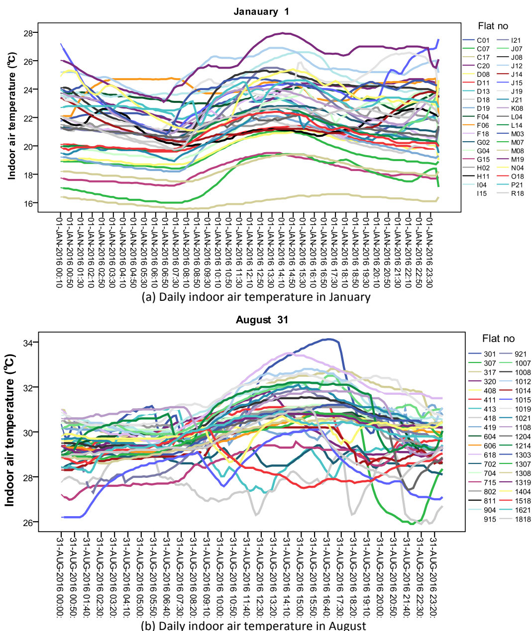
Figure 9 Daily indoor air temperatures of winter and summer months.
