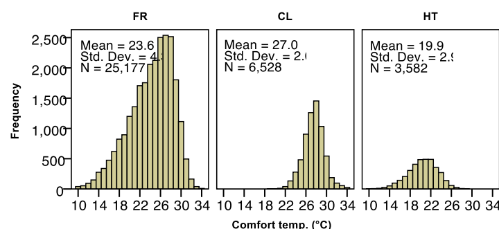
Figure 8. Estimation of comfort temperatures from each observation by Griffiths' method.
