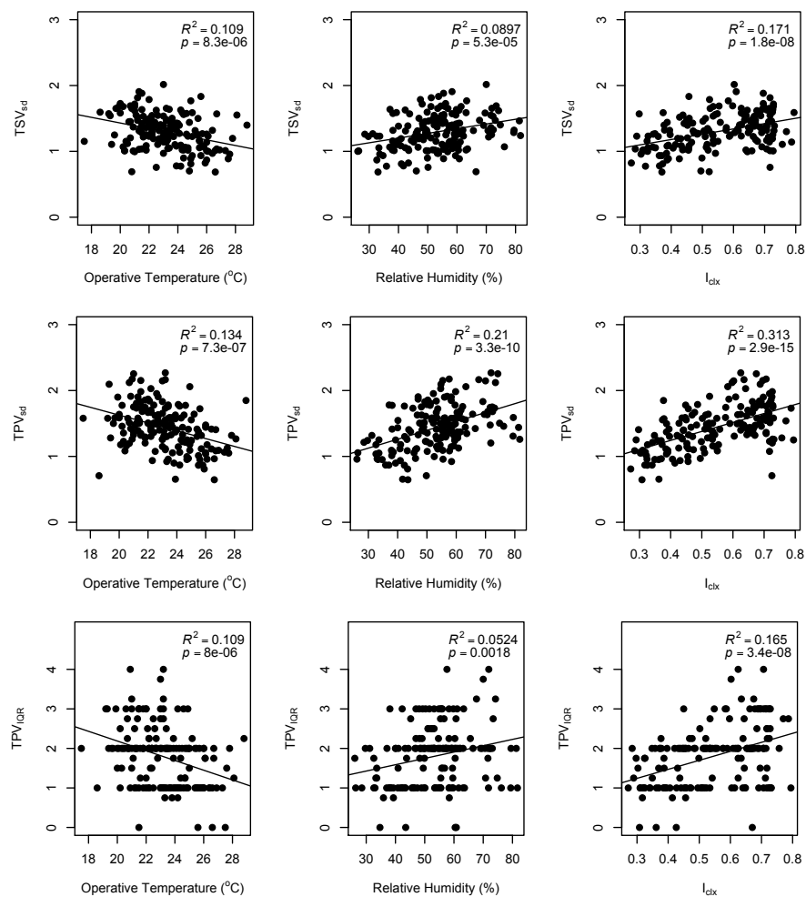
Figure 5. Relationship between [operative temperature, relative humidity and mean clothing insulation] and [ TSV_{sd} , TPV_{sd} and TPV_{IQR} ] during the non-heating season at survey level
