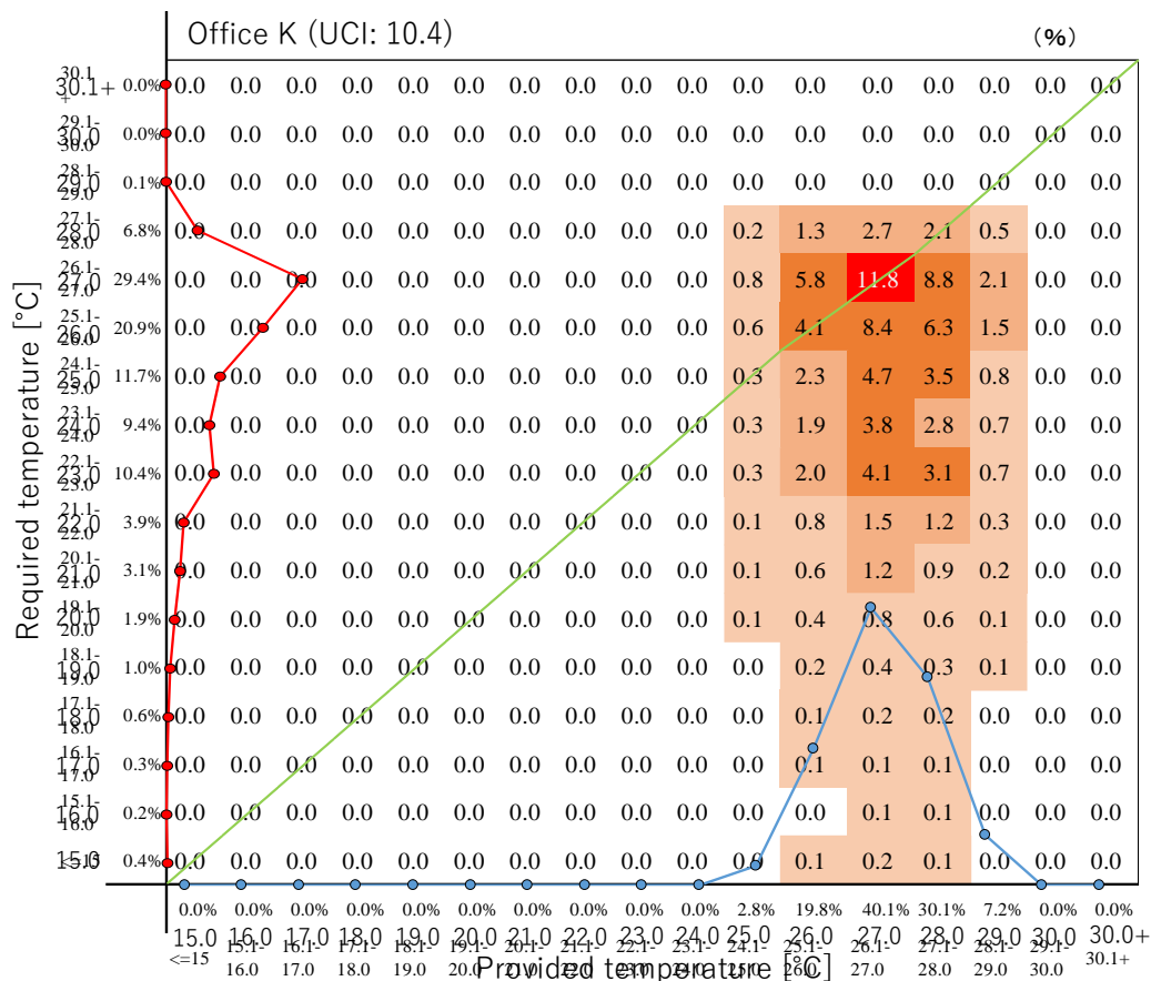
Figure 16. Result of P-R chart for office K (convective air-conditioning system)
