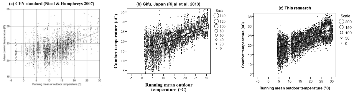
Figure 13. Variation of the comfort temperature in previous and this research.
