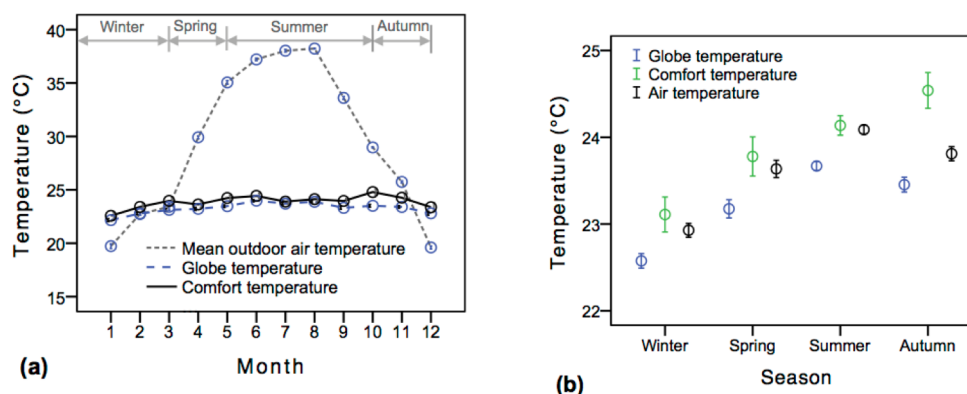
Figure 11 (a). Monthly and (b). seasonal variations in outdoor temperatures and the corresponding indoor and comfort temperatures. Error bars indicate 95% CI.
