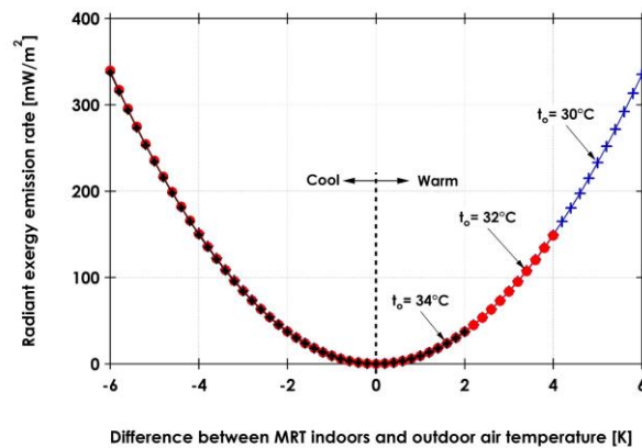
Figure 8. Radiant exergy as a function of surface temperature. A surface, whose temperature is higher than the environmental temperature, emits “warm” radiant exergy and lower emits “cool” radiant exergy.
