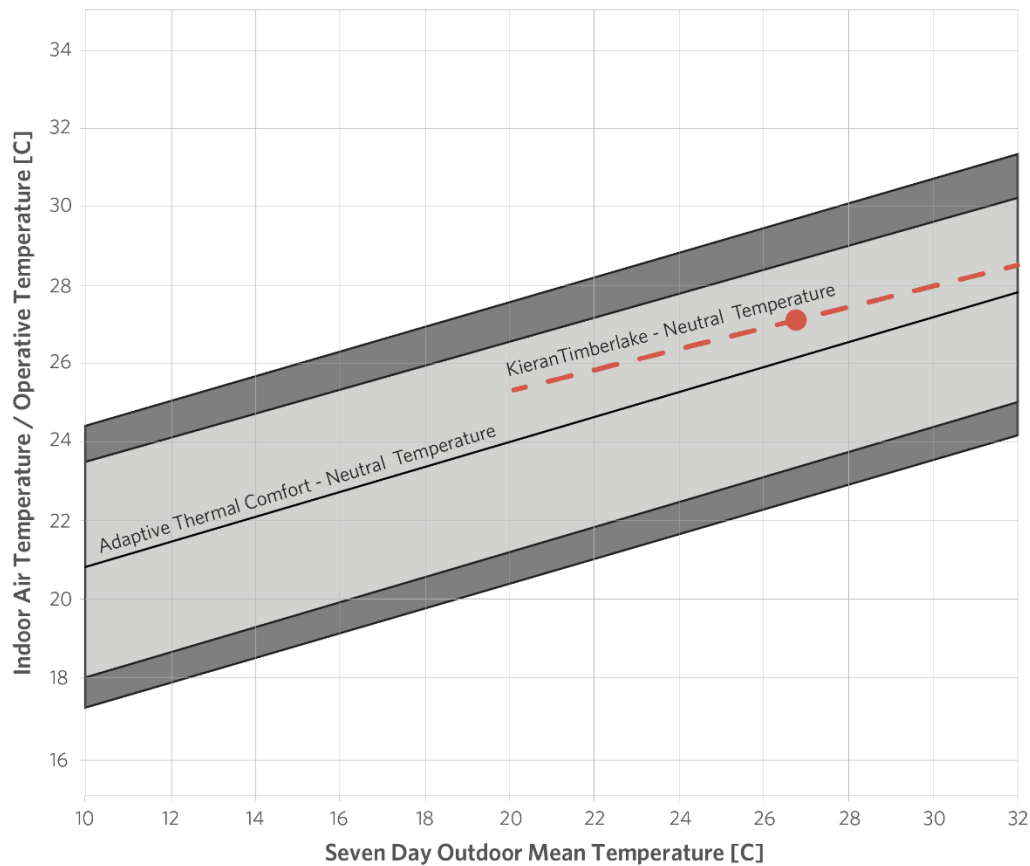
Figure 8: A graph plotting the optimal indoor temperature for a range of outdoor prevailing mean temperatures showing the study's comfort limits are approximately 1.0-1.8 °C greater than the adaptive thermal comfort model.
