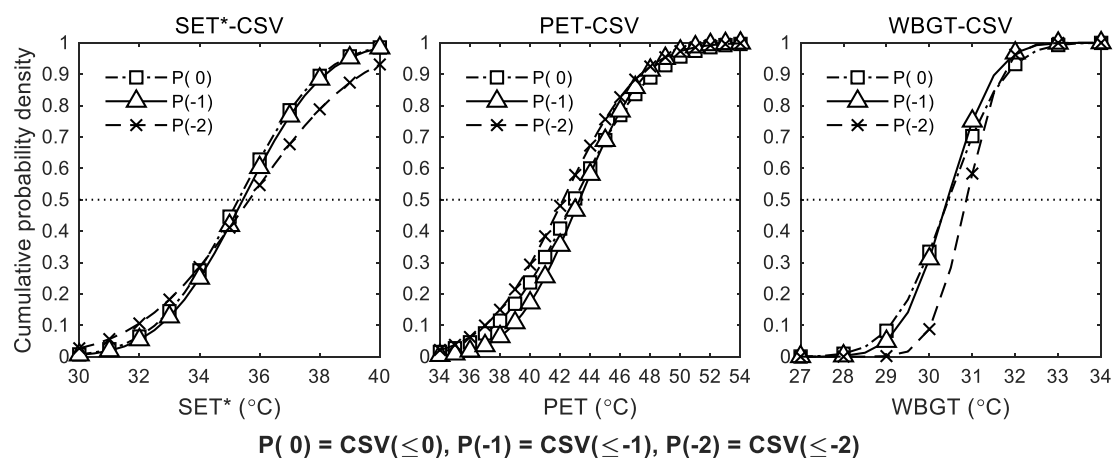
Figure 6. Correlation of CSV and each thermal index calculated by the measurement results.
