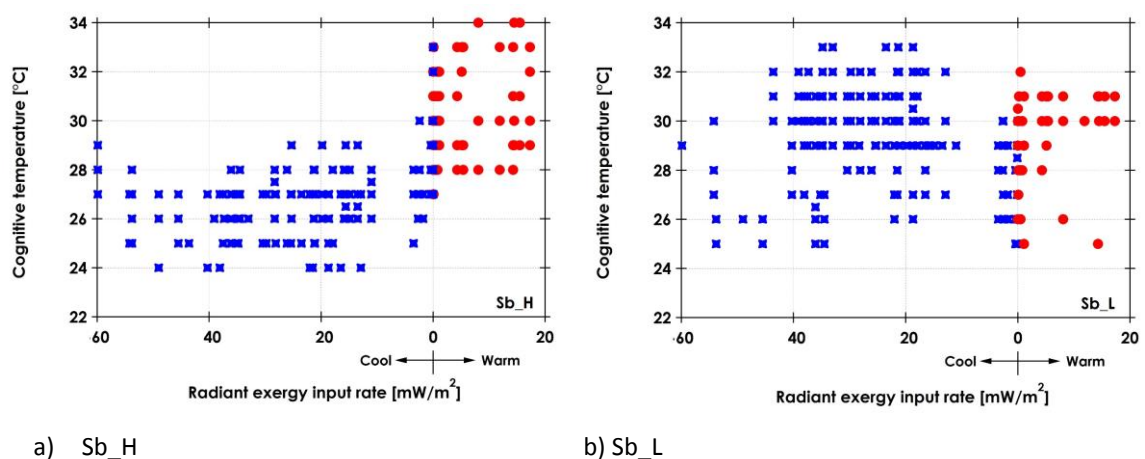
Figure 7. Cognitive temperature and its relation to radiant exergy input rate
