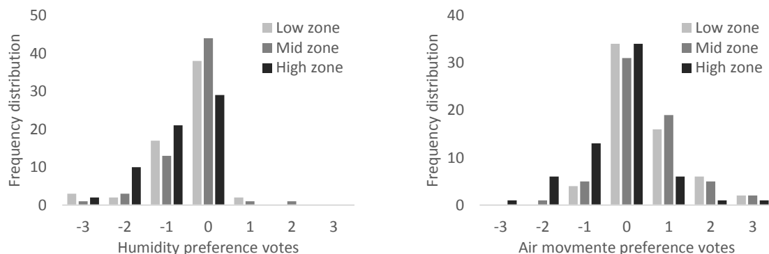
Figure 9: Distribution of humidity and air movement preference votes
