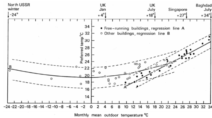
Figure 2. Correlation between the neutral temperatures against the mean monthly temperature of the exterior (Humphreys et al, 2016)
