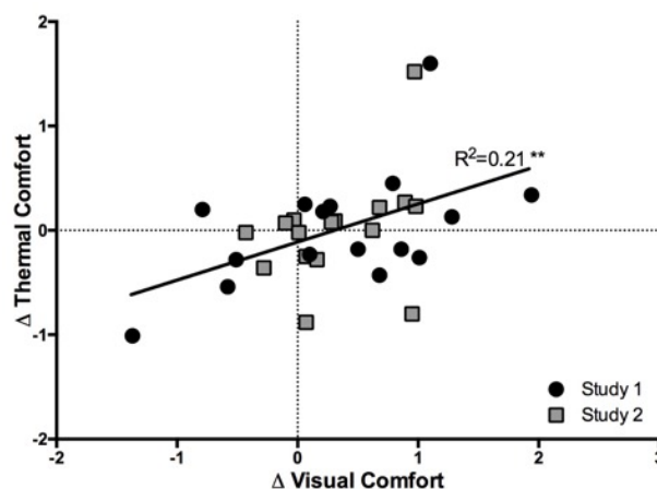
Figure 5 \Delta Visual Comfort & \Delta Thermal Comfort during the cool condition between each participants' two light exposures either \Delta_{\text{bright-dim}} for study 1 (black dots) or \Delta_{2700\text{K}-6500\text{K}} for study 2 (grey squares).
