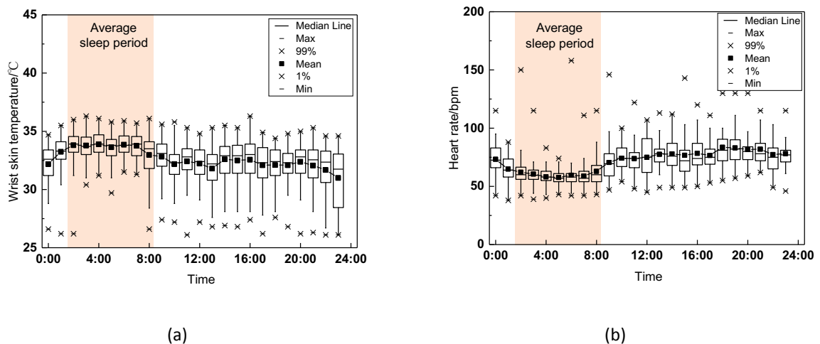
Figure 5. Physiological parameters. (a) Wrist skin temperature. (b) Heart rate.
