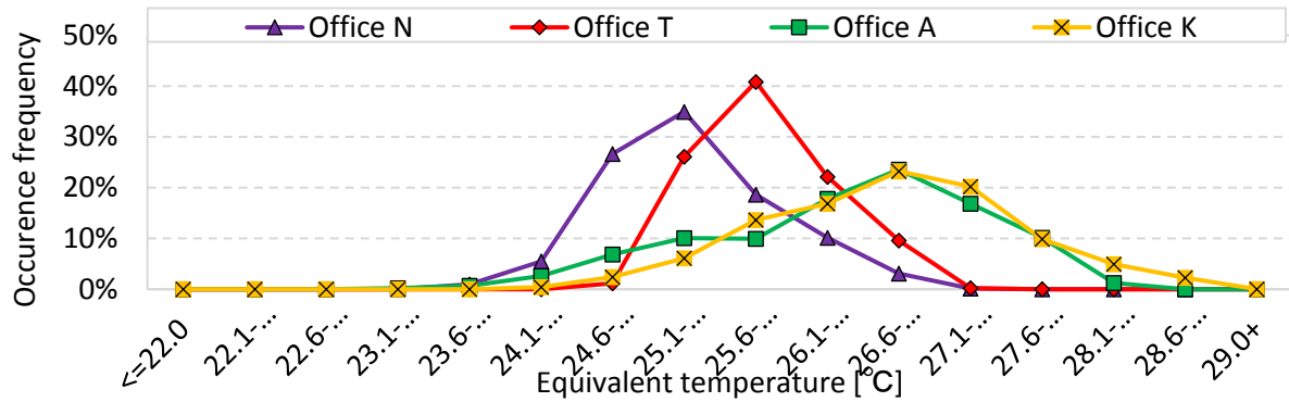
Figure 10. Occurrence frequency of equivalent temperature
