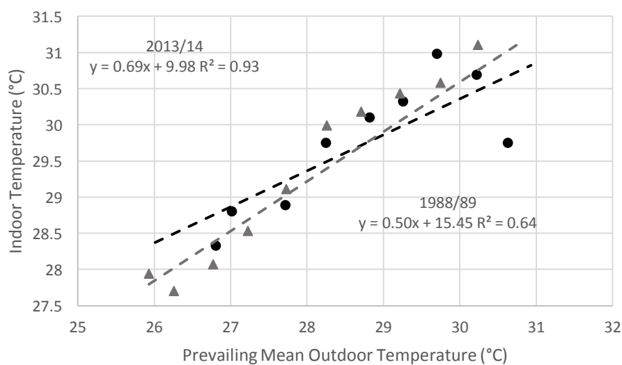
Figure 12. Plot of Prevailing outdoor versus Internal temperature at time of TSV voting
