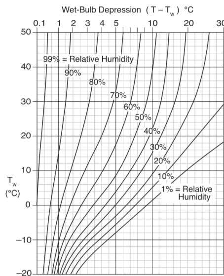
Figure 1. A psychrometric chart for the standard pressure of 101.325 kPa at sea level showing the changes scale for wet-bulb temperature ( T_w ) and relative humidity (Stull, 2011).
