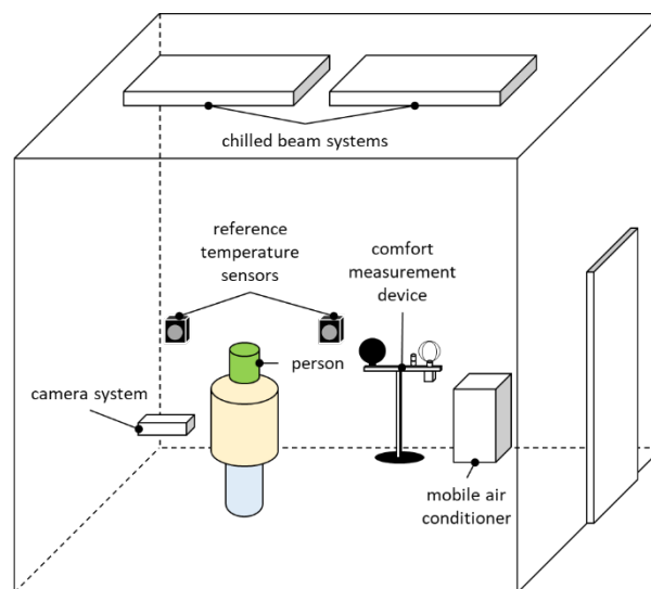
Figure 6. Schematic of the entire experimental setup, redrawn from (Metzmacher et al., 2017)
