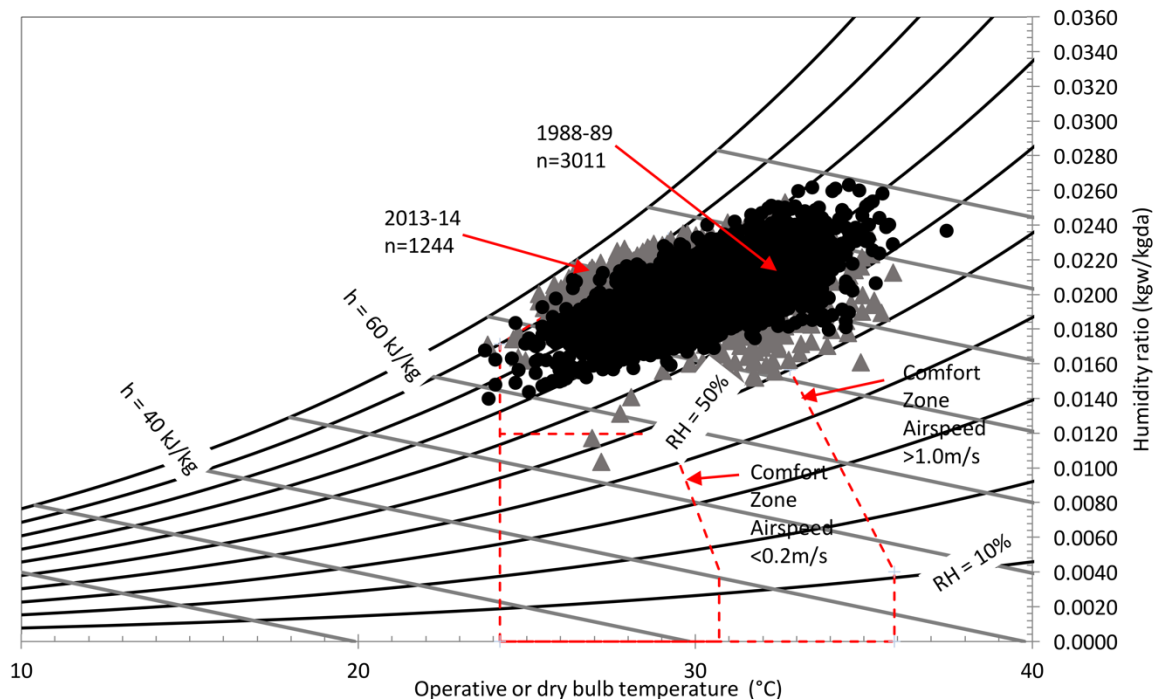
Figure 6. Indoor environmental conditions at the times that thermal comfort vote surveys were completed compared with the ASHRAE 55-2013 acceptable comfort zone for conditioned spaces (0.5 & 1.0 clo zones combined)
