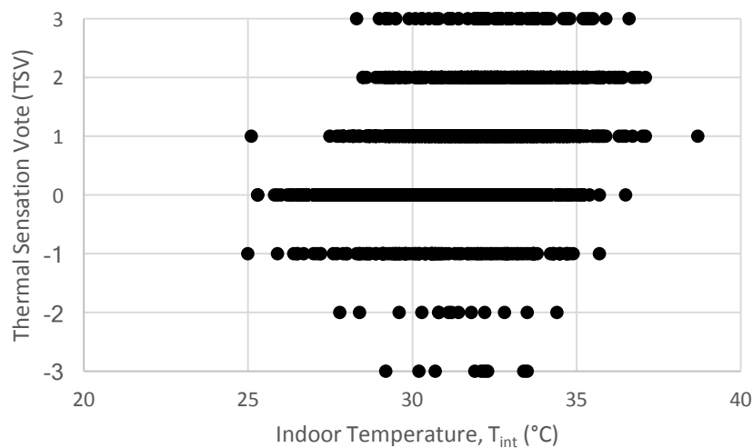
Figure 11. Thermal Sensation Votes vs Indoor Temperature, 1988/89 Study
