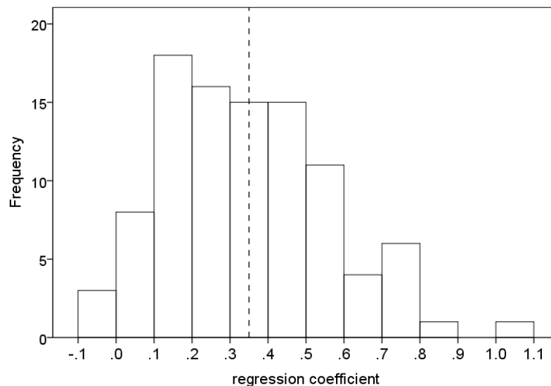
Figure 2. Histogram of regression coefficients ( N \geq 50 ). (source: Humphreys et al 2016)
