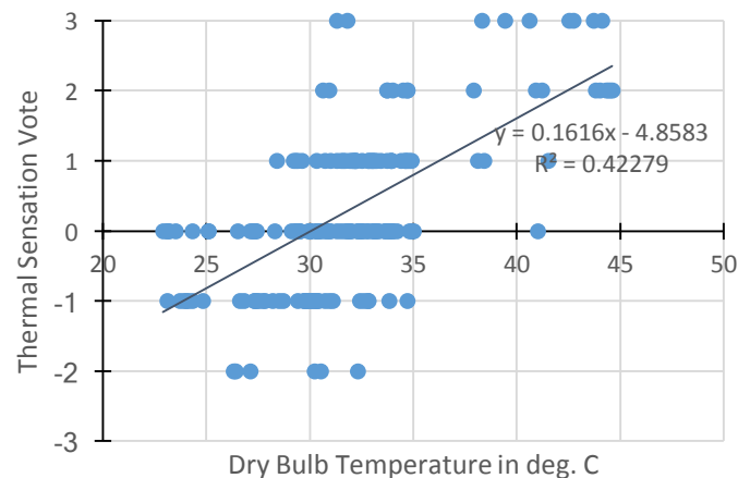
Figure 18 Correlation between the thermal sensation vote and dry bulb temperature
