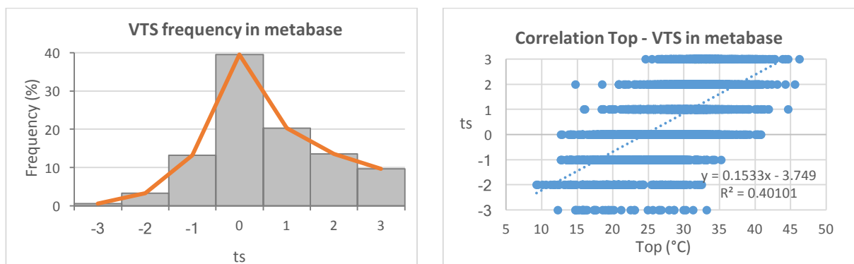
Figure 11. Histogram and scatter diagram in metabase
