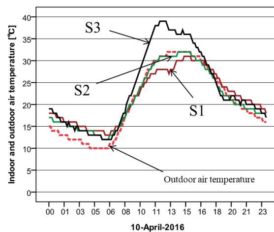
Fig. 6 Variation of indoor and outdoor air temperature in a day in summer
