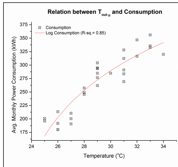
Figure 6: Relation between T_{out-\mu} and energy consumption
