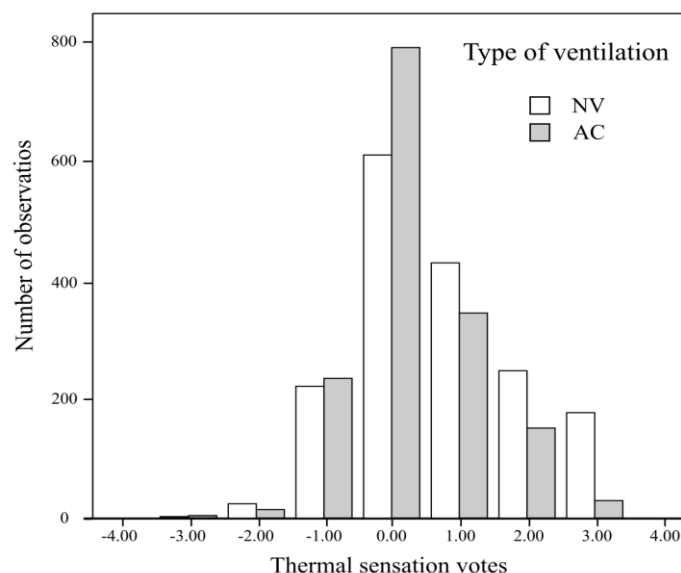
Figure 2. Distribution of thermal sensation votes in NV and AC mode
