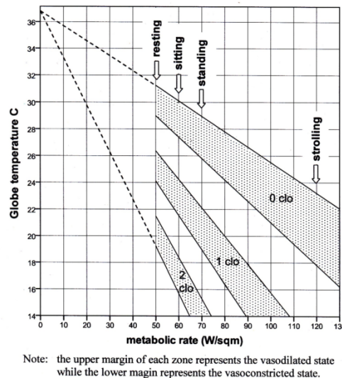
Figure 2, Humphreys 1979 schematic diagram of comfort zoned for still air and various levels of clothing (from Humphreys et al 2016 chapter 20)
