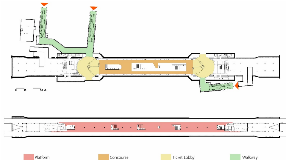
Figure 2 Identified zones in the metro station floor plan
