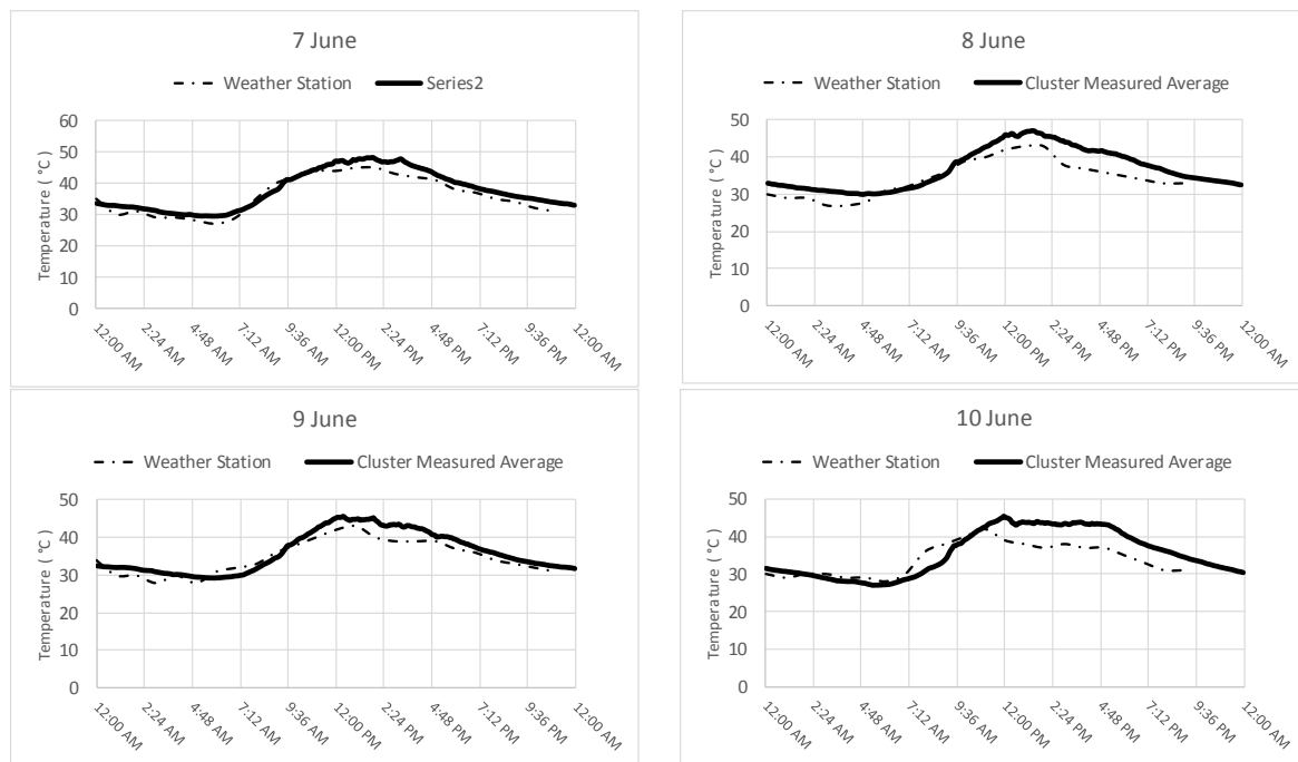
Figure 7. Comparison between the measured temperatures at the cluster and the temperatures recorded at Al Maktum weather station
