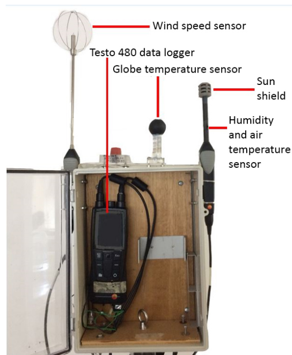
Figure 2 Set up of microclimatic measurement station
