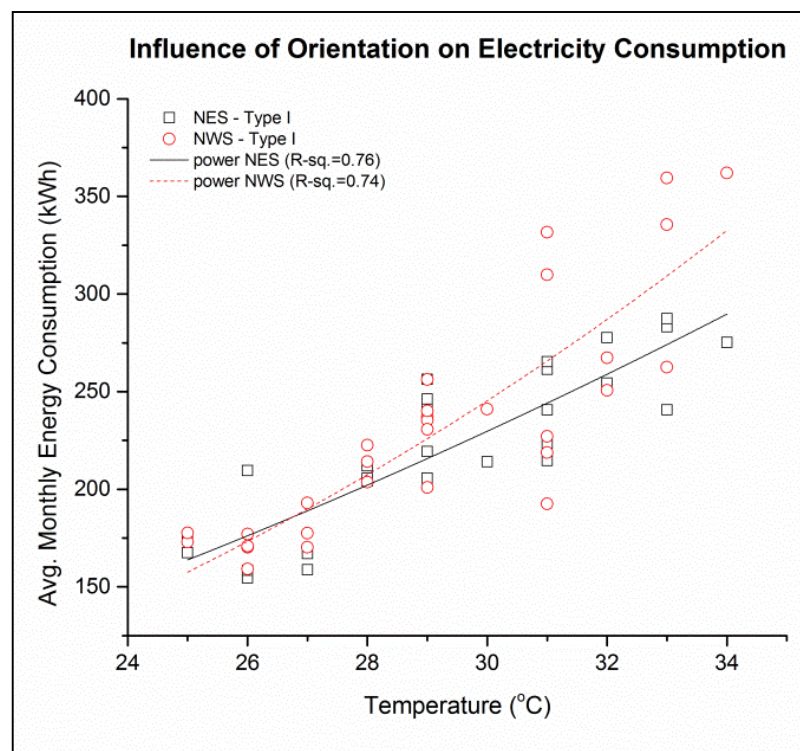
Figure 10 (b): Influence of orientation on operational energy consumption
