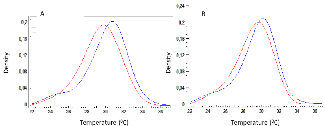
Figure 4: Comparison of density traces of summer temperature distributions (°C) for dwellings without cooling systems (blue line) compared to dwellings with cooling equipment (red line) during the day from 8 a.m. to 11 p.m. (a) and at night from 11 p.m. to 8 a.m. (b).
