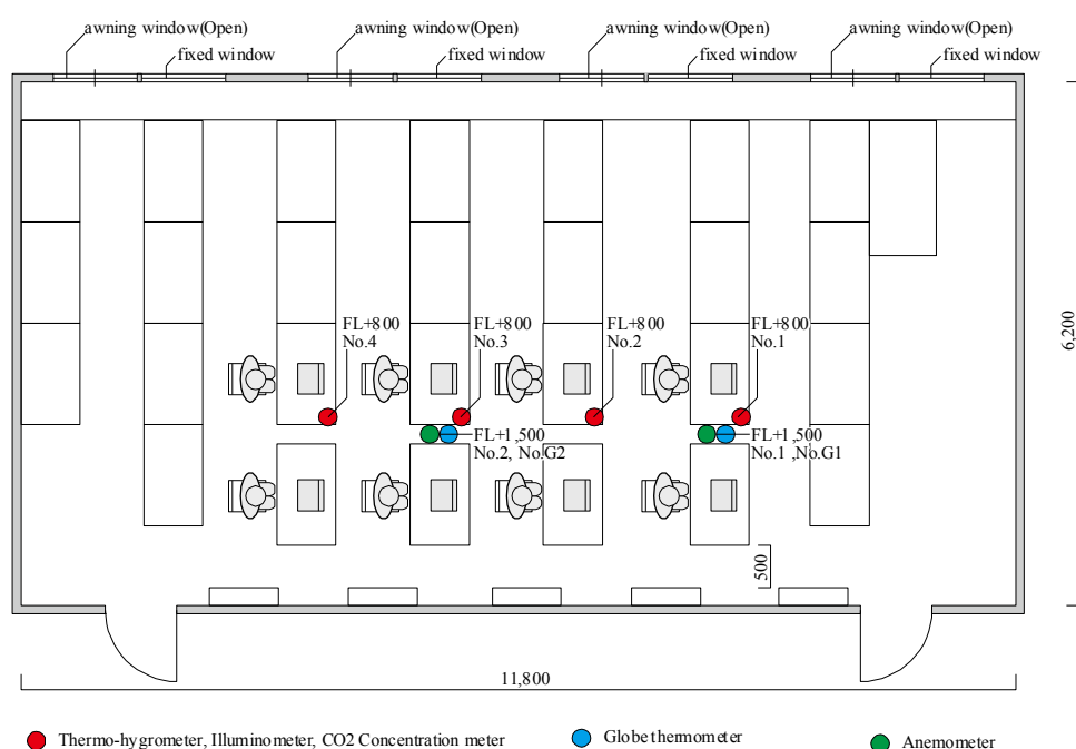
Figure 1. Plan of experimental room and positions of physical measurements
