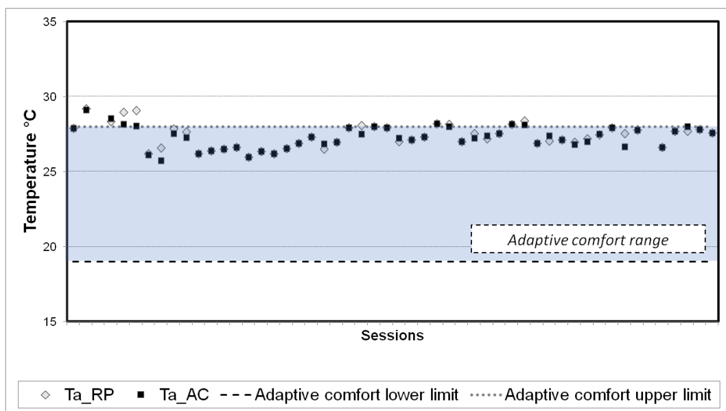
Figure 5 – Air temperature conditions in both rooms during the 53 sessions
