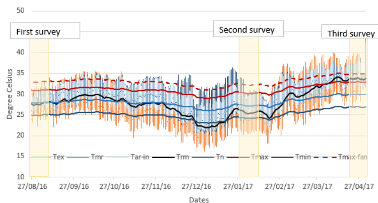
A - AKTH temperature time series
