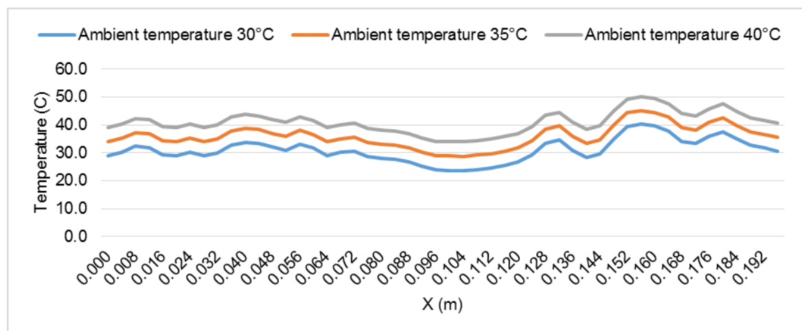
Figure 14. Temperature profiles along the axial direction of the cluster
