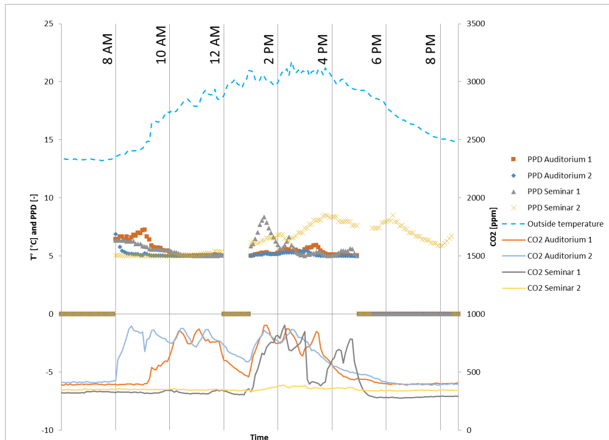
Figure 3. Typical day results (29 th September 2016) : CO 2 level, PPD computation and outside t°
