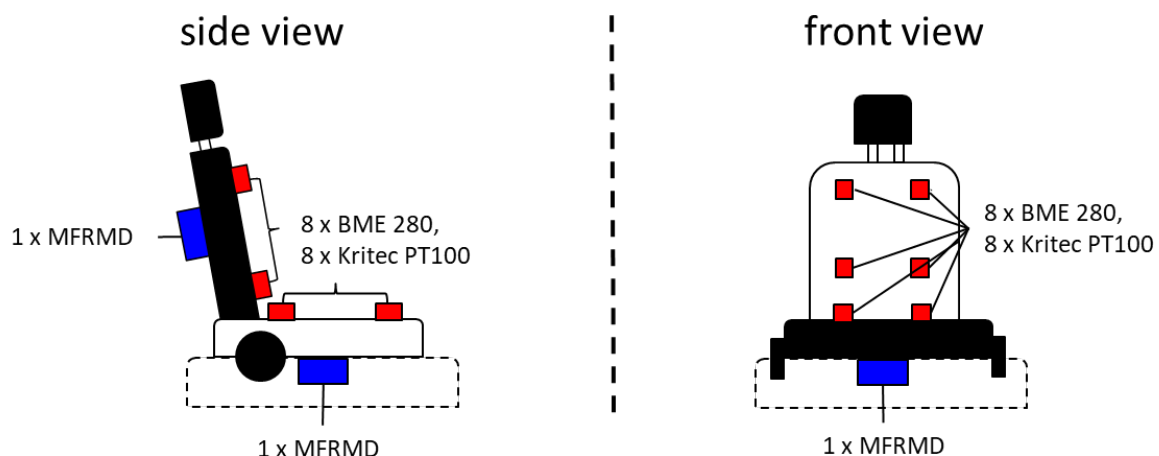
Figure 4: Schematic of the a seat, equipped with the corresponding measurement devices; BME 280: humidity and temperature sensor, Kritec PT100: temperature sensor, MFRMD: in-house developed sensor for the measurement of the mass flow rate delivered by the fans, mounted at the backside of the backrest and the backside of the cushion
