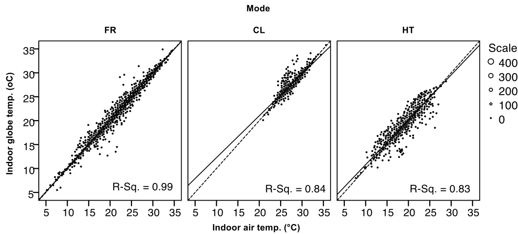
Figure 4. Relation between the indoor globe temperature and indoor air temperature.
