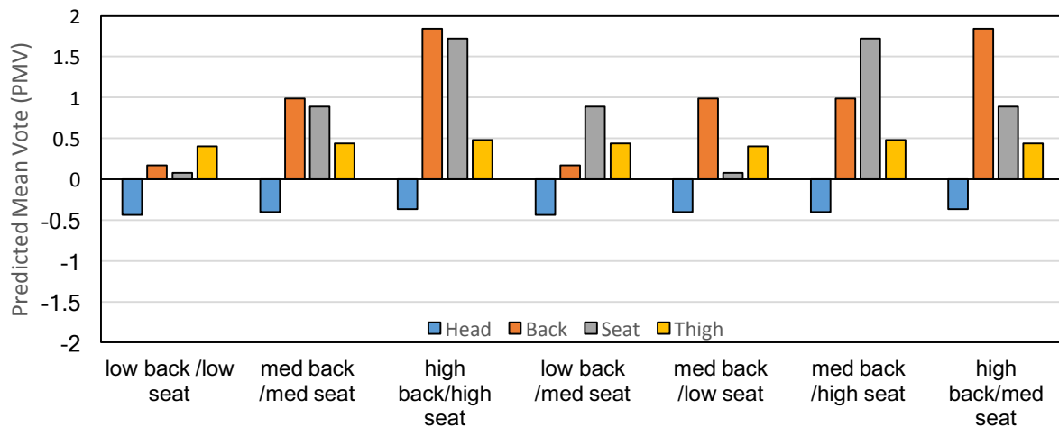
Figure 4. Effect of varying the seat and back settings (low, medium and high) on Predicted Mean Vote at different locations.
