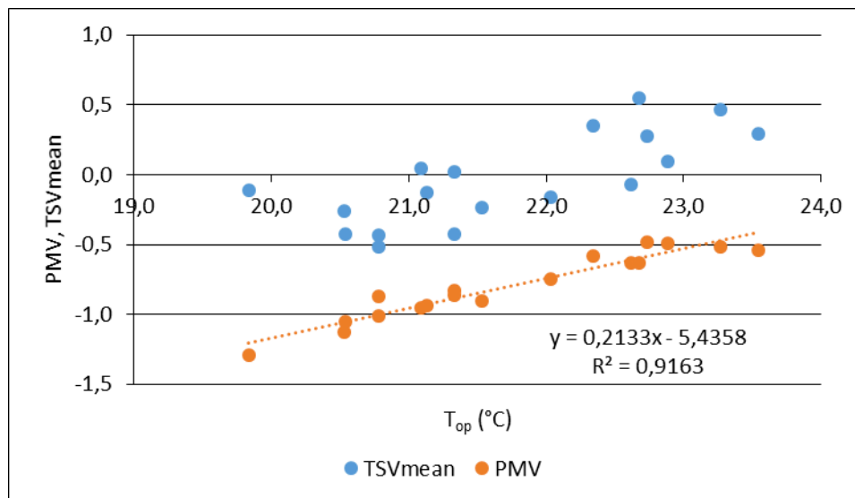
Figure 6. Relationship between mean TSV, predicted mean vote (PMV) and operative temperature
