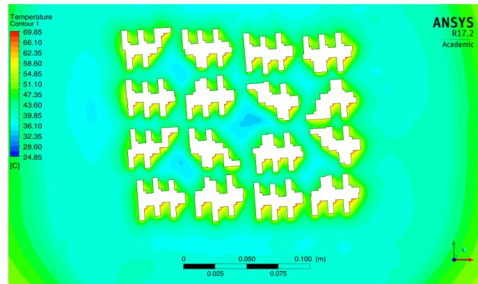
Figure 13. Plan view of the temperature contour levels
