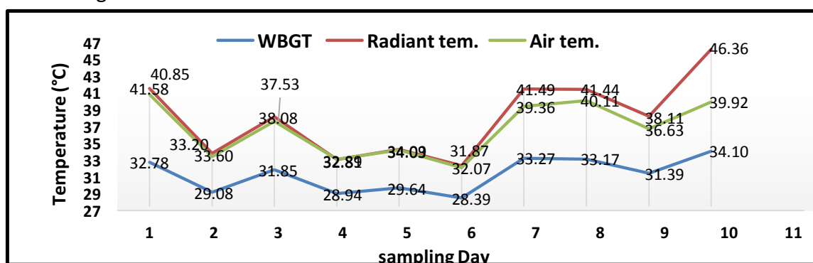
Figure 2: Mean WBGT, radiant temperature and air temperature during the field study
