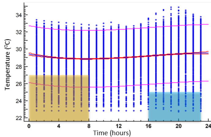
Figure 5: Distribution of daytime temperatures (°C) in the summer months in the group of dwellings compared to Cooling setpoint temperatures, in accordance with to the Energy Rating procedure and characterisation of CTE-HE demand. Night temperature setpoint (ochre) and afternoon temperature setpoint ( blue).
