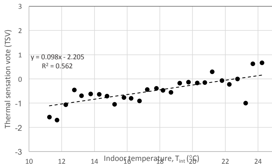
Figure 5: Weighted regression of thermal sensation vote and indoor temperature binned in 0.5K intervals
