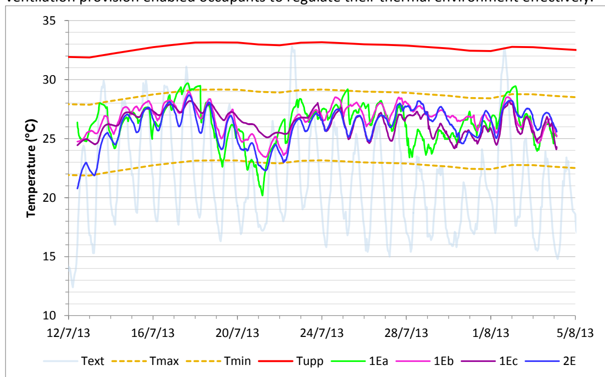
Figure 7: Internal temperatures in rooms on first and second floor between 12 th July and 4 th August, showing the Cat II adaptive thermal comfort thresholds (Tmax and Tmin) and the CIBSE TM52 Criterion 3 upper limit temperature (Tupp)
