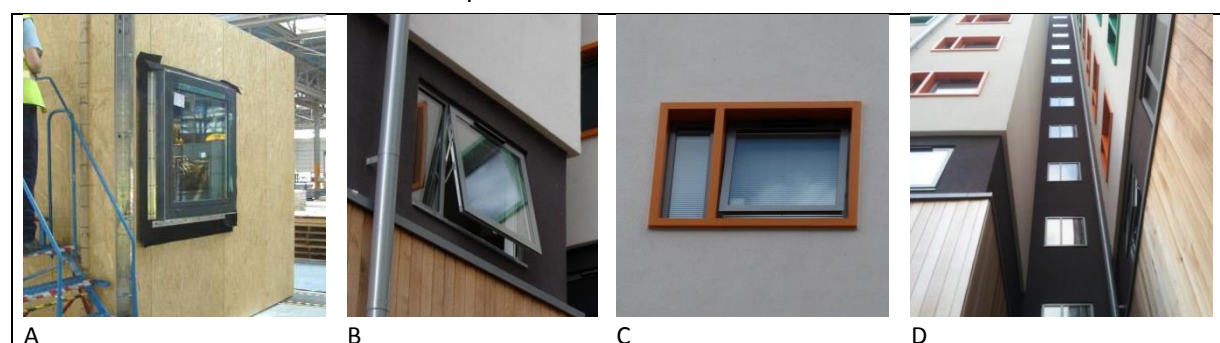
Figure 4: Window in bedroom module, not recessed in facade (A), Bedroom window recessed in facade showing the extent of window opening (B), Bedroom window in planar facade— extent of window opening (C), Stair core, fixed, opaque windows with large bedroom windows left & right (D)
