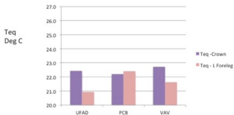
Fig 12 Teq Deg C Crown & L Foreleg – Thermal Manikin - Clothing value = 0.36 – Uncovered legs
