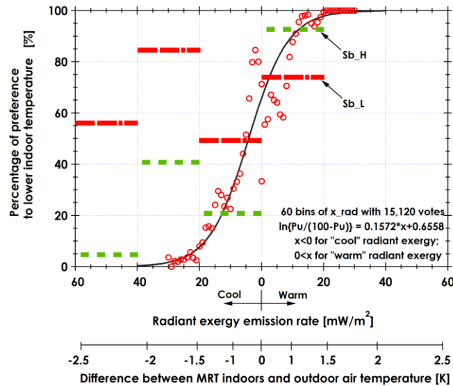
Figure 9. The relationship between radiant exergy emission rate from the surrounding surfaces and the percentage of subjects who prefer lowering the room temperature
