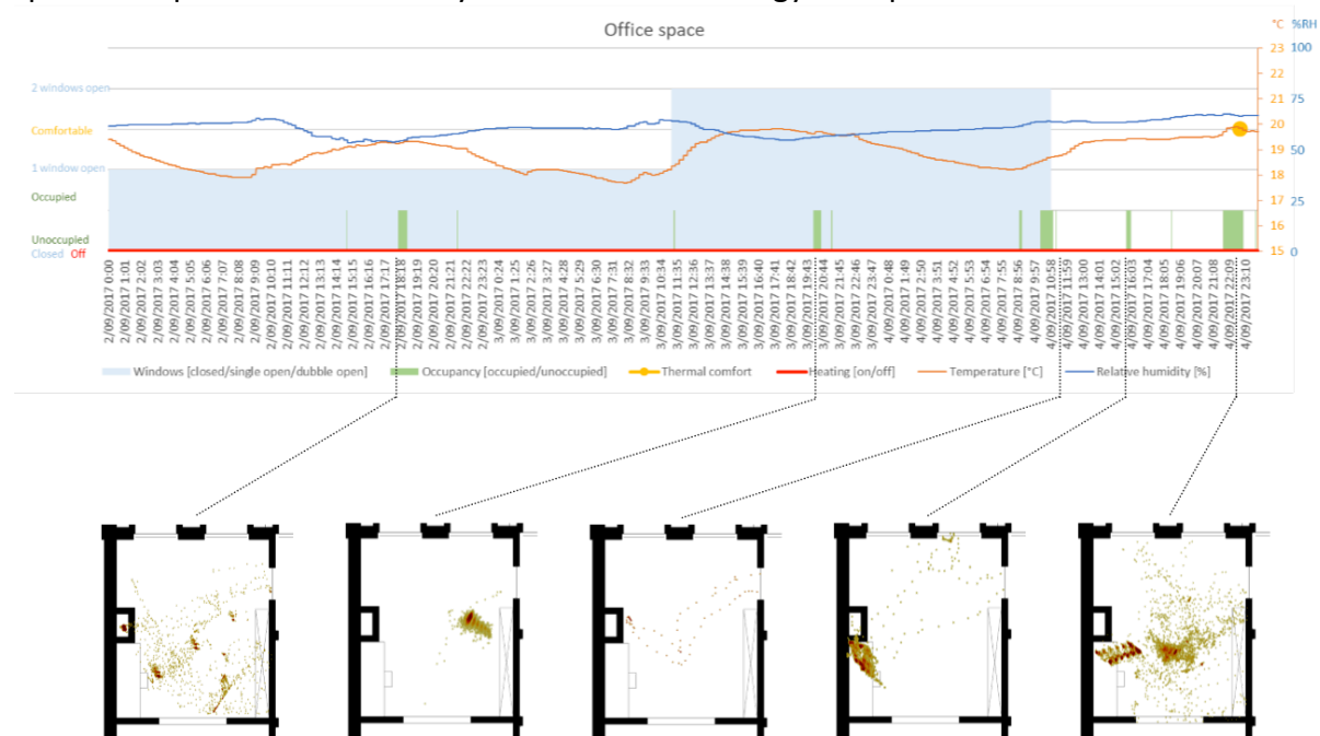
Figure 6: Timeline during 3 days from resident 2 in the office space of dwelling 2: combined data on occupation, actions, indoor climate, comfort experience and spatial use
