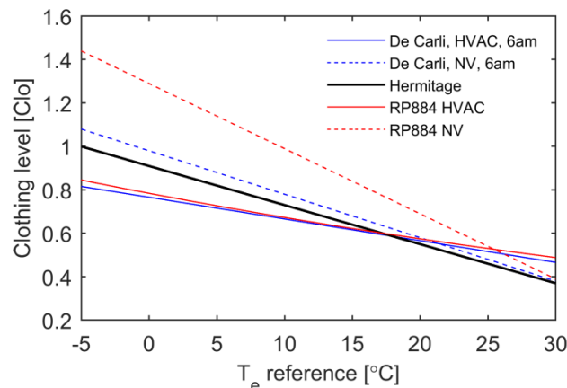
Figure 7. Clothing level as a function of reference outdoor temperature according to De Carli et al. (De Carli et al. 2007), ASHRAE RP884 (de Dear & Brager 1998), and experimental data from the Hermitage Amsterdam museum (R. P. Kramer et al. 2017).
