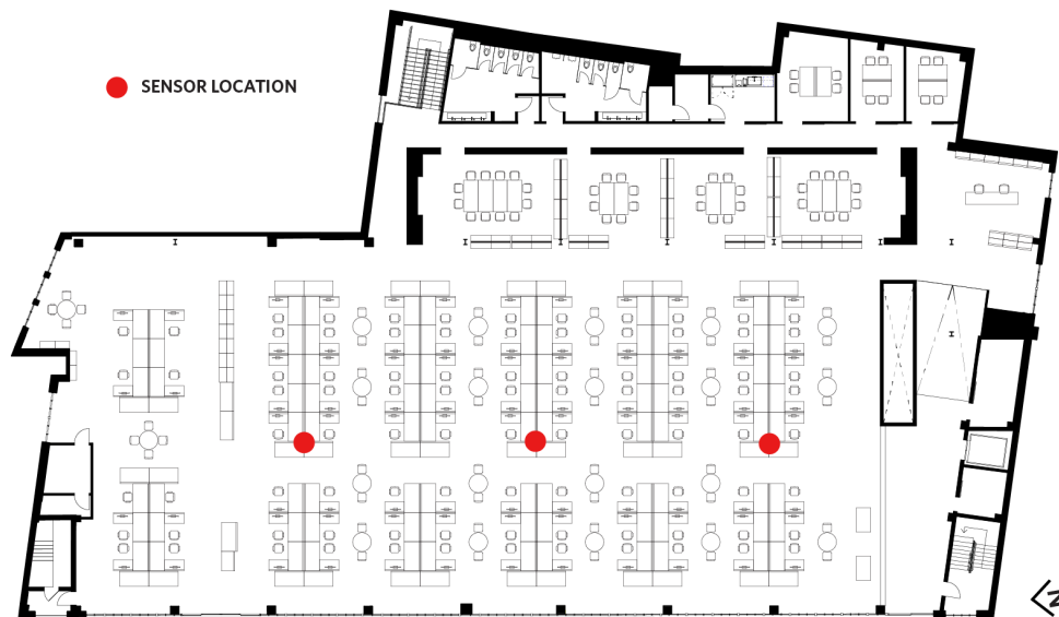
Figure 3: Floor plan of the office showing location for the three ambient temperature and humidity sensors, mounted at 1.1 meters above the finished floor.
