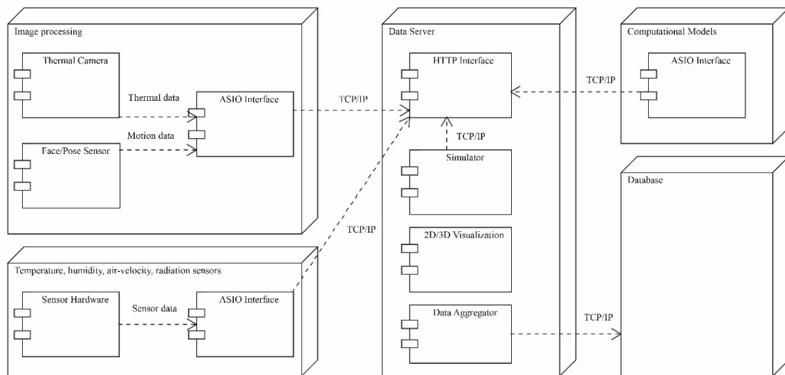
Figure 1. Overview of the system architecture. The system is designed around a central data server which handles communication and data storage (Metzmacher et al., 2017b)
