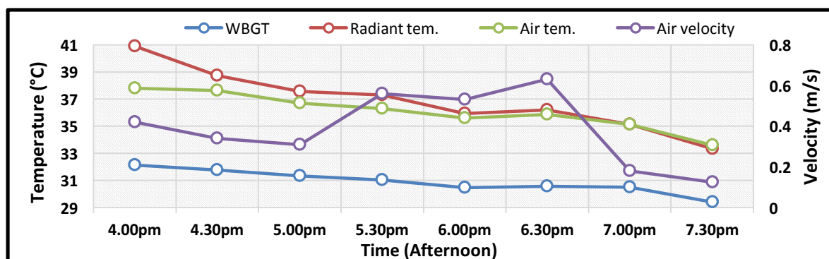
Figure 3: The average decreasing trend of three Environmental parameters related to human thermal response (WBGT, Radiant temperature and Air temperature) and air velocity over sampling time (afternoon).
