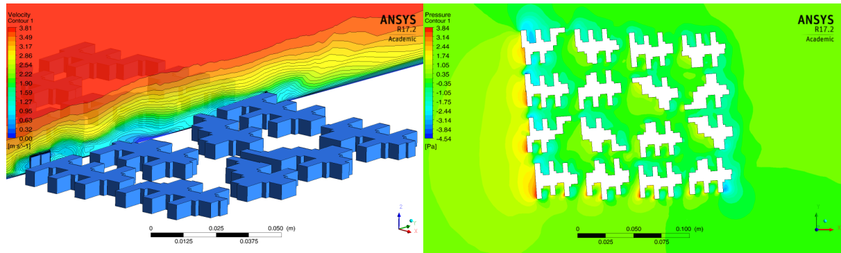
Figure 12. (a) Velocity and (b) static pressure contour levels across the cluster
