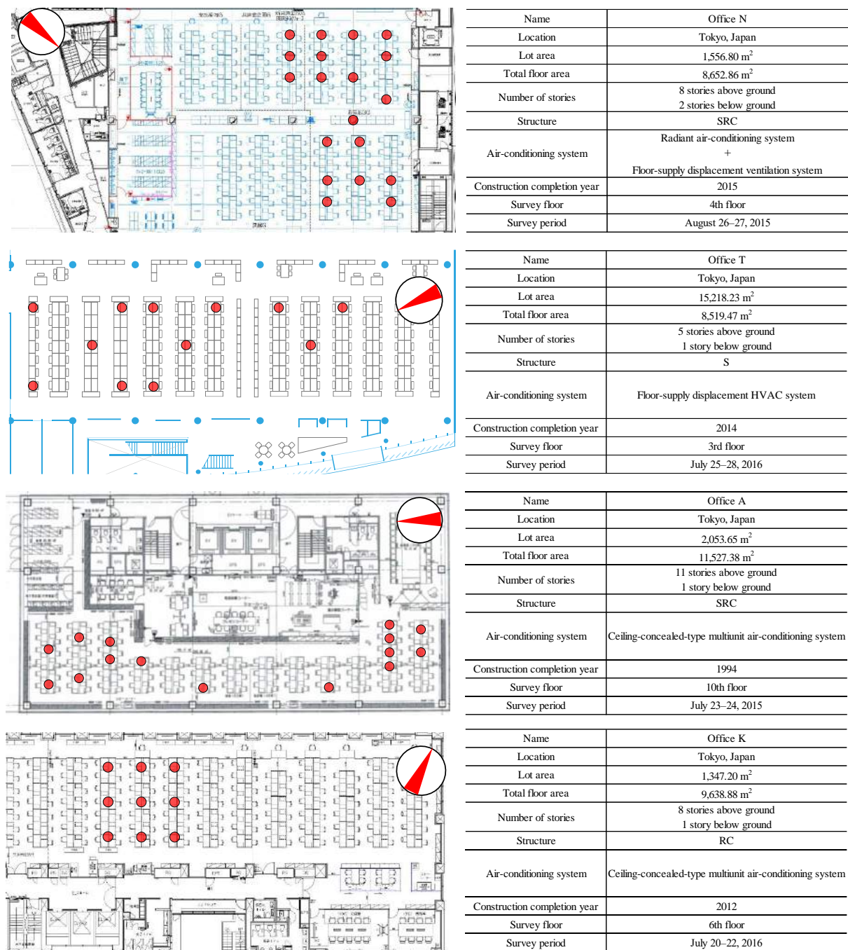
Figure 5. Floor plan and thermal measurement points for each office
