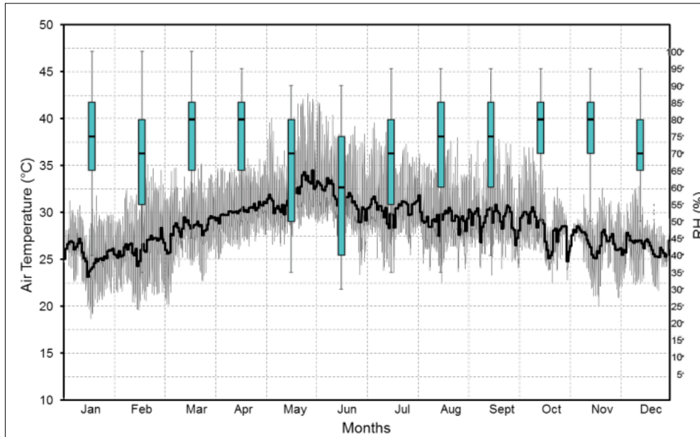
Figure 1: Summary of climatic conditions
