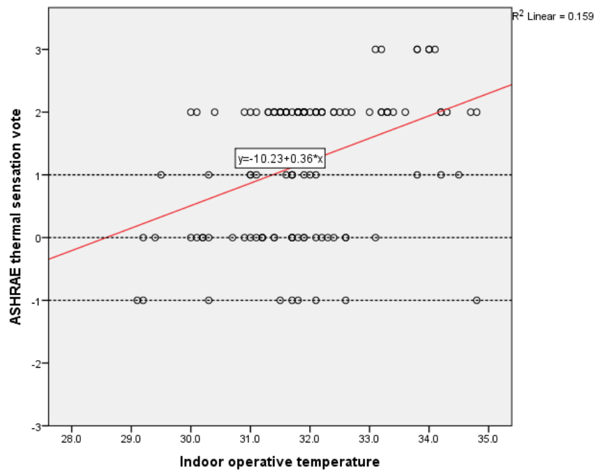
Figure 7. Linear regression of indoor operative temperature and ASHRAE sensation votes
