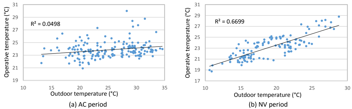
Figure 4. Outdoor temperatures plotted against indoor operative temperature (Top), for AC and NV periods
