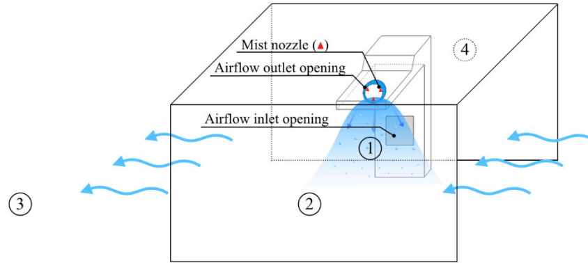
(e) Mist system concept and the location of measurements
