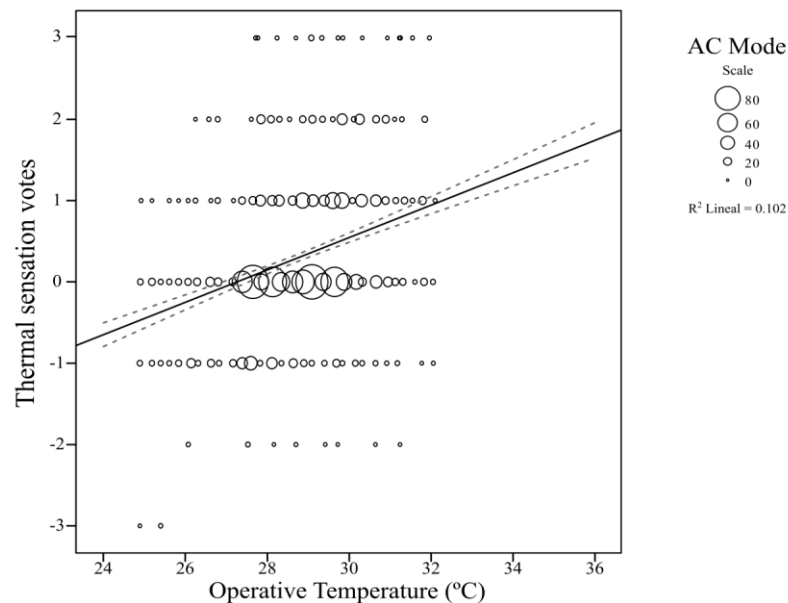
Figure 6. Linear regression of thermal sensation votes and operative temperature ( T_{op} ) in AC mode
