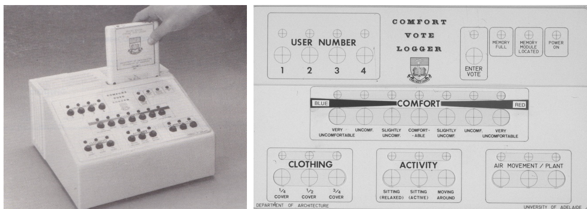
Figure 2. Comfort Vote Logger and detail of front panel
