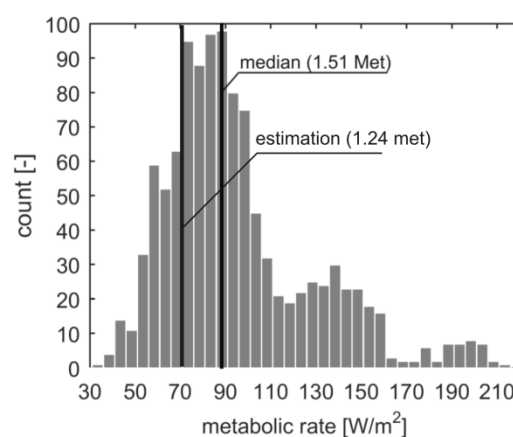
Figure 8. Comparing the a priori estimated metabolic rate with the metabolic rate identified from experimental data (R. Kramer et al. 2017).
