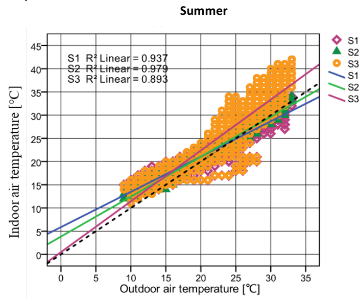
Fig. 7 Relationship between indoor and outdoor air temperature of three shelters in summer
