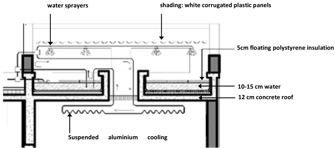
Figure 2 – Configuration 6 of the Roof Pond, with permanent spraying and water circulation in the ceiling radiative panels
