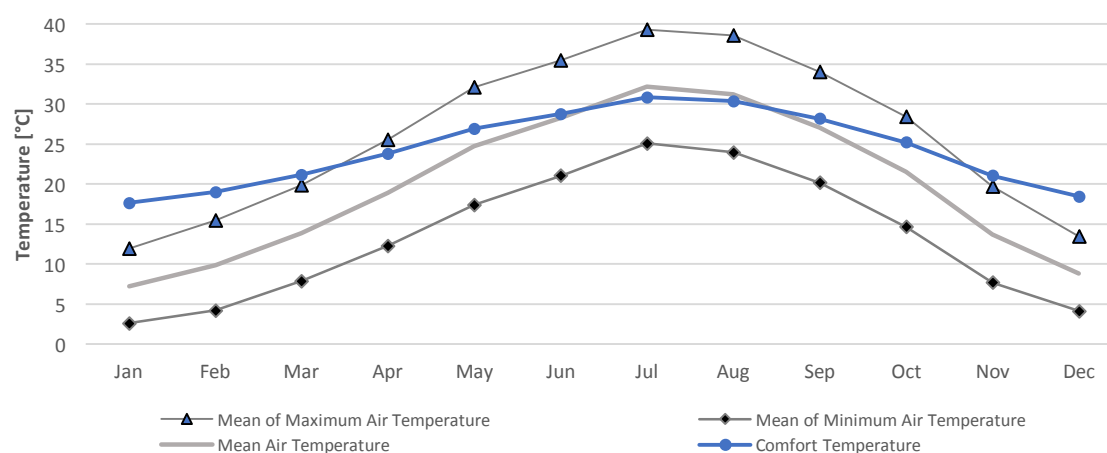
Figure 6: Nicol Graph for Baghdad based on Meteonorm climate data
