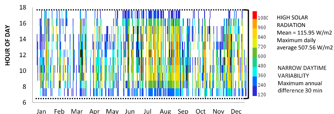
Figure 3: Quito global normal radiation (W/m 2 ) – Source: NREL
