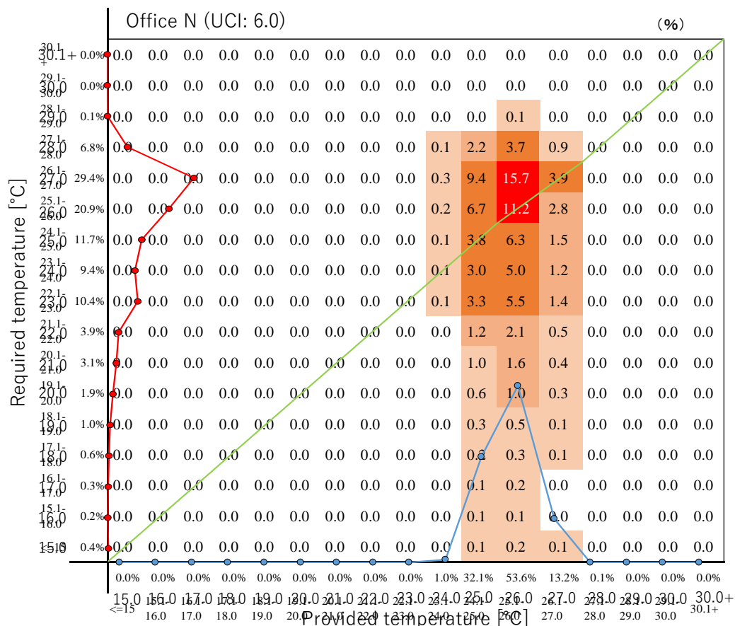
Figure 13. Result of P-R chart for office N (radiant air-conditioning system)
