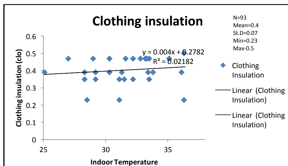
Figure 3.2: Scatter plots of clothing insulation and temperature
