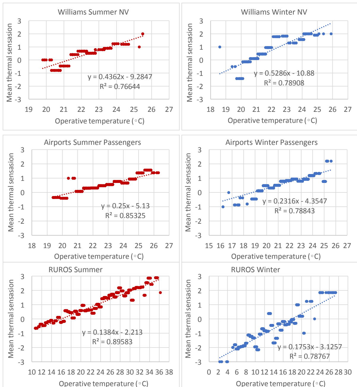
Figure 4: Mean thermal sensation as a function of operative temperature (°C) for the different studies
