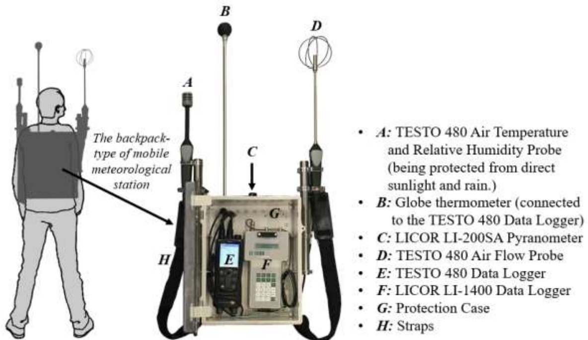
Figure 3. Instrumental settings of the mobile meteorological station.
