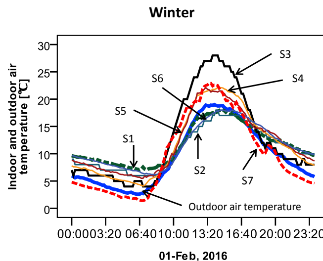
Fig. 5 Variation of indoor and outdoor air temperature in a day in winter
