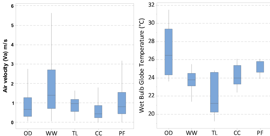
Figure 8 Air velocity and wet bulb globe temperature at different zones of metro station
