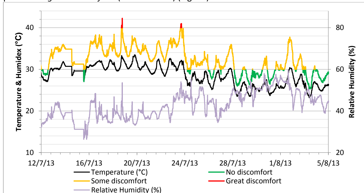
Figure 10: Humidex rating and measured temperature and relative humidity for room 10Wa between 12 th July to 4 th August
