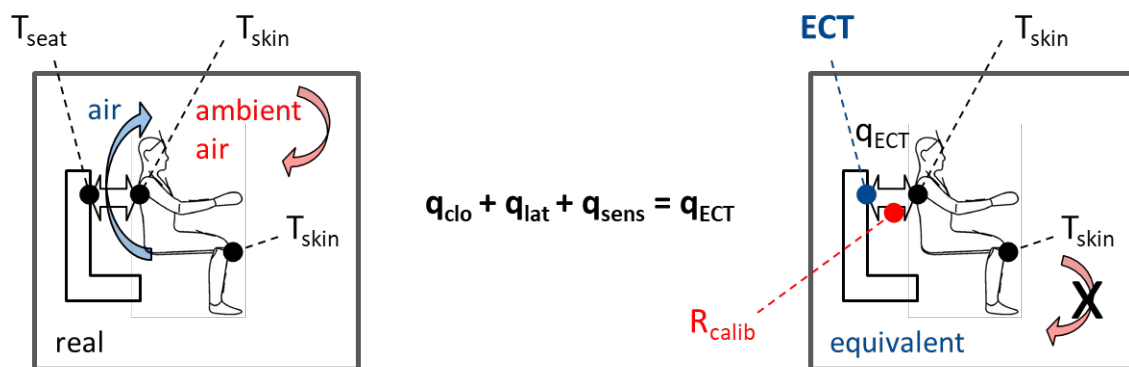
Figure 1. Definition and physical interpretation of the equivalent contact temperature (ECT); left-hand side: non-uniform situation, right-hand side: uniform equivalent; T_{\text{seat}} : seat surface temperature [°C], T_{\text{skin}} : local skin temperature [°C], v_{\text{air}} : air speed at the contact interface [m/s], ECT: equivalent contact temperature [°C], q_{\text{clo}} : heat flux density through clothing [W/m²], q_{\text{lat}} : latent heat flux density caused by evaporation of sweat [W/m²], q_{\text{sens}} : sensible heat flux density at the contact interface [W/m²], q_{\text{ECT}} : equivalent heat flux density [W/m²].
