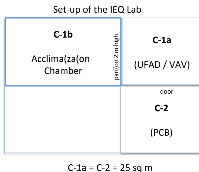
Figure 4. Chamber 1 sub-division C-1a & C-1b & Chamber 2, C-2
