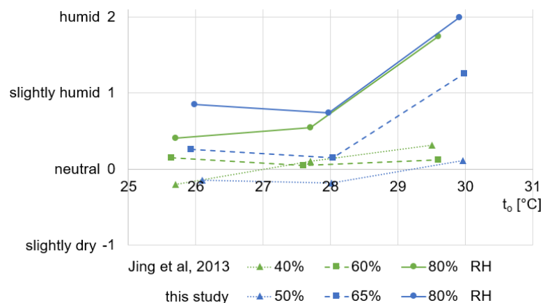
Figure 7. Comparison of humidity sensation (HSV) in relation to operative temperature in this study and the study of (Jing et al, 2013)
