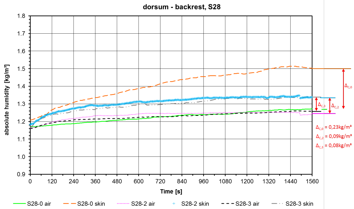
Figure 10: Transient behaviour of the absolute humidity at the contact interface between the dorsum and the backrest of the seat; S28-0 to S28-3: test scenarios for 28 °C and fan levels of 0 %, 65 % and 100 %
