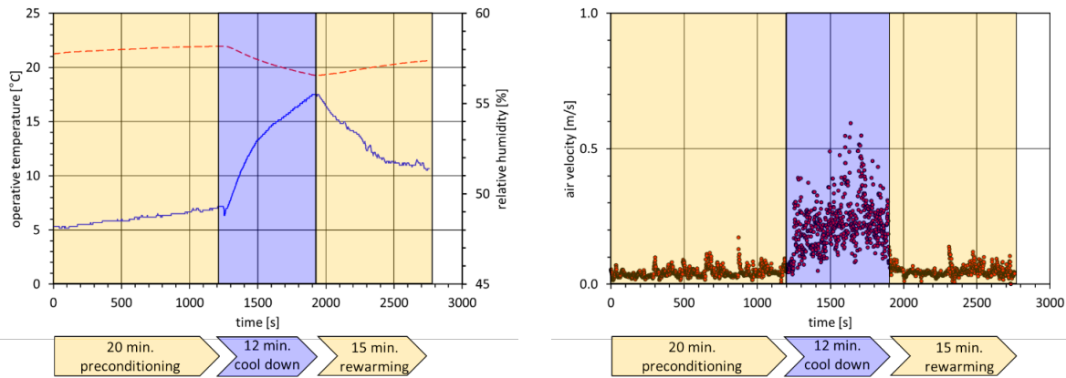
Figure 7. Boundary conditions of the experiment measured at a height of 1.2 m above the floor; dashed line left-hand side: operative temperature ( T_{op} ), solid line left-hand side: relative humidity ( rh ), right-hand side: average air velocity ( v_{air} )
