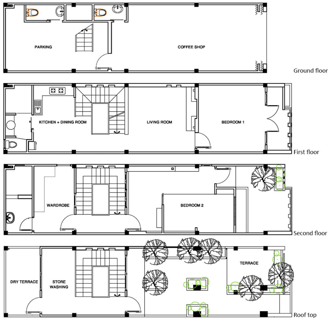
Figure 2. An example of a new shophouse in HCMC – No 6, Street No 41, District 4
