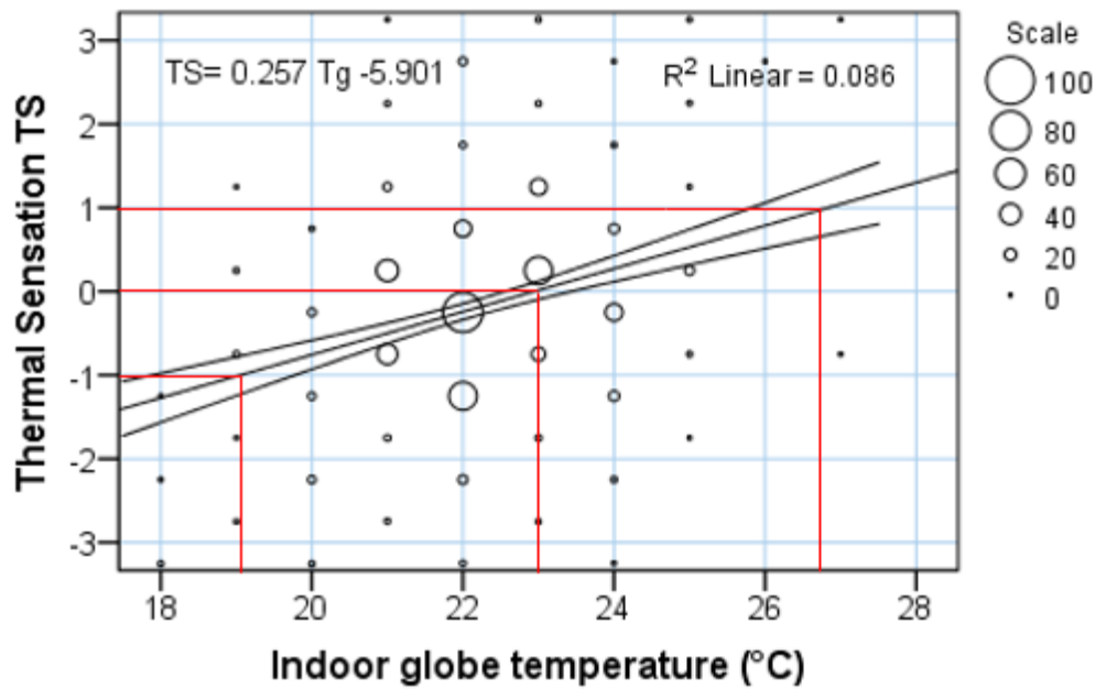
Figure 29. Relationship between indoor globe temperature and thermal sensation.
