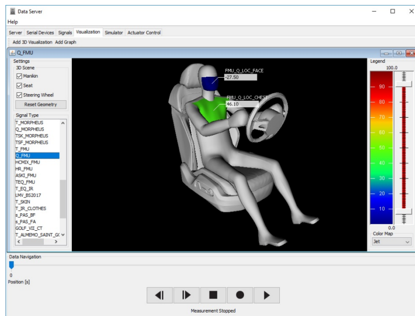
Figure 4. 3D visualization of energy surpluses and requirements at the individual's head and chest region respectively.
