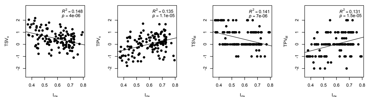
Figure 4. Relationship between mean clothing insulation and [ TSV_{\bar{x}} , TPV_{\bar{x}} , TSV_M and TPV_M ] in the UK at survey level
