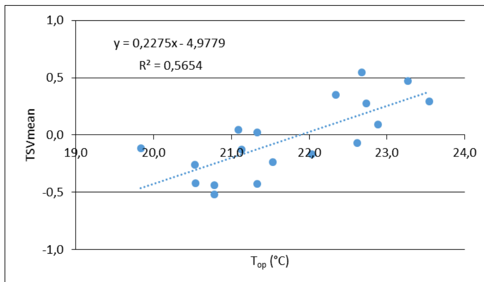
Figure 5. The relationship between mean thermal sensation vote ( TSV_{mean} ) and the operative temperature
