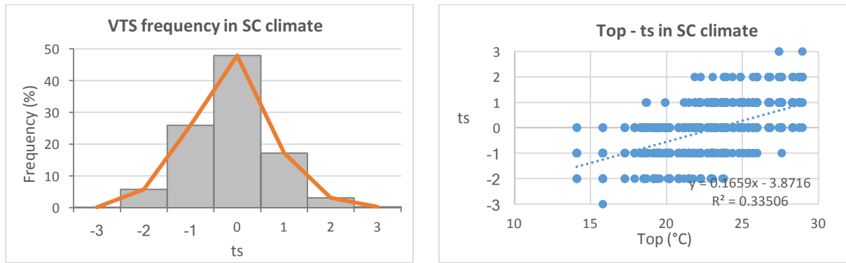
Figure 8. Histogram and scatter diagram in SC climate
