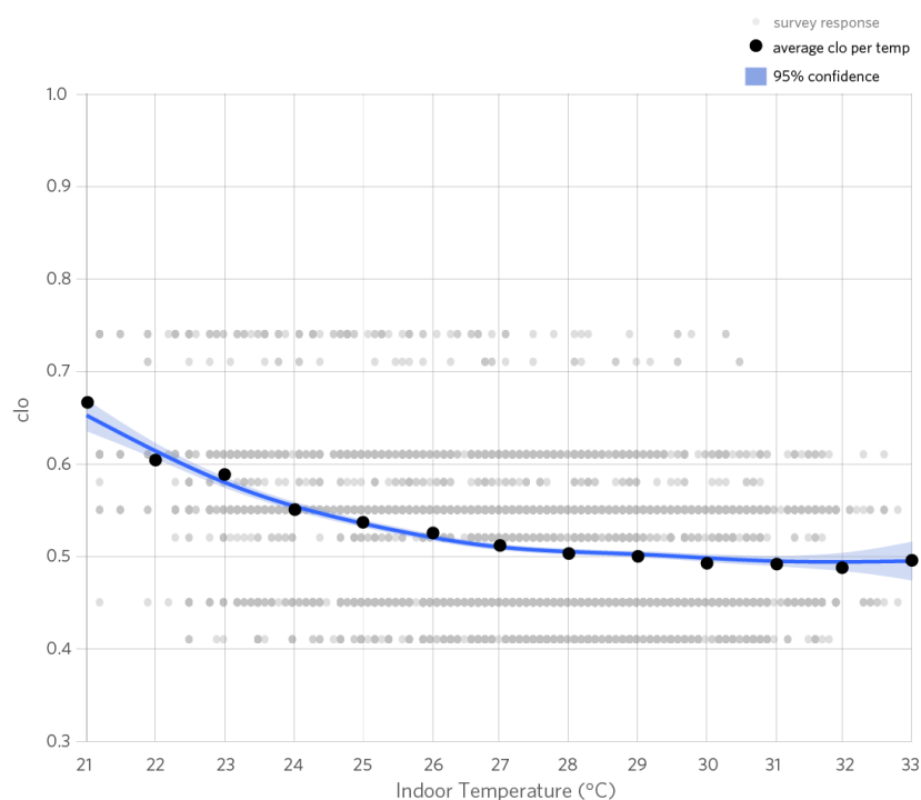
Figure 7: The average clo values decrease until temperatures reach 27 °C. At temperatures above 27 °C, clo values reach a steady minimum value of 0.50.
