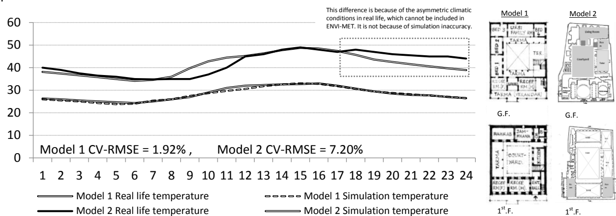
Figure 3. The comparison between courtyard houses' real and simulation temperature (left), and the plans of the used Baghdadi courtyard houses (right).
