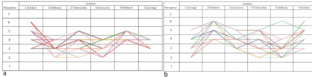
Figure 13 Thermal perception during winter performing (a) boarding and (b) alighting
