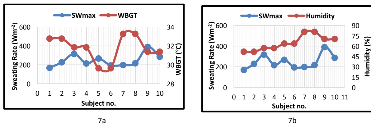
Figure 7: Maximum sweating rate relation to WBGT (7a) and humidity (7b).
