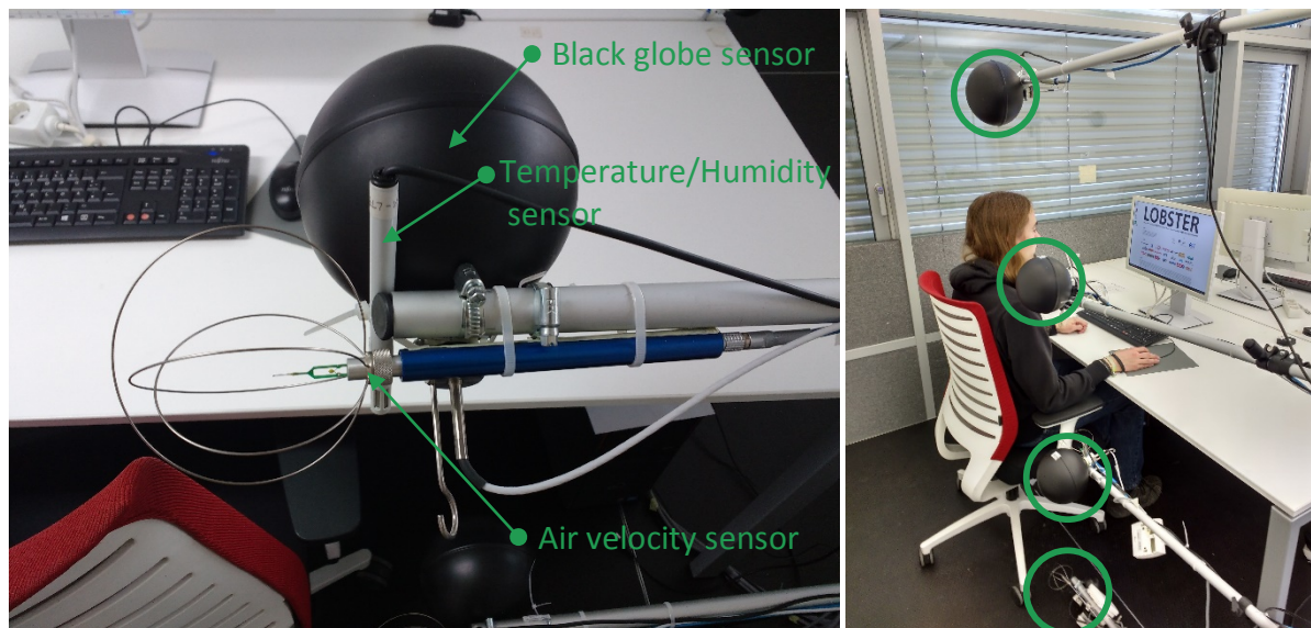
Figure 4: Sensors (air temperature/humidity, air velocity and globe temperature) and their positions at 10, 60, 110 and 170 cm from the floor
