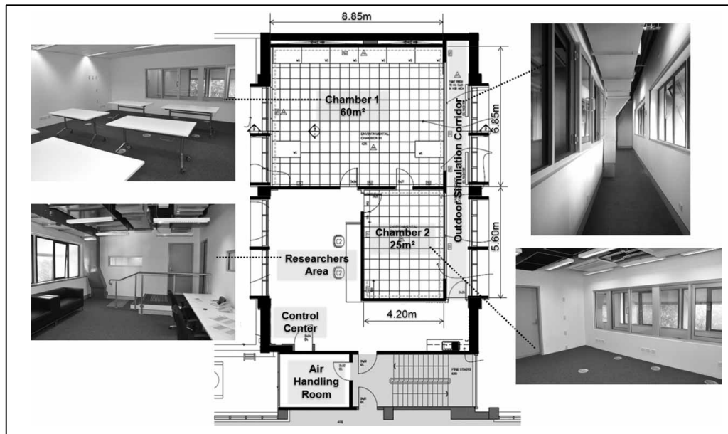
Figure 2. Climate Chambers & Associated Spaces
