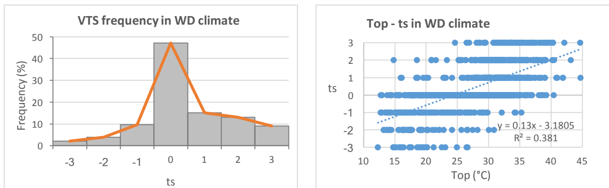
Figure 9. Histogram and scatter diagram WD climate
