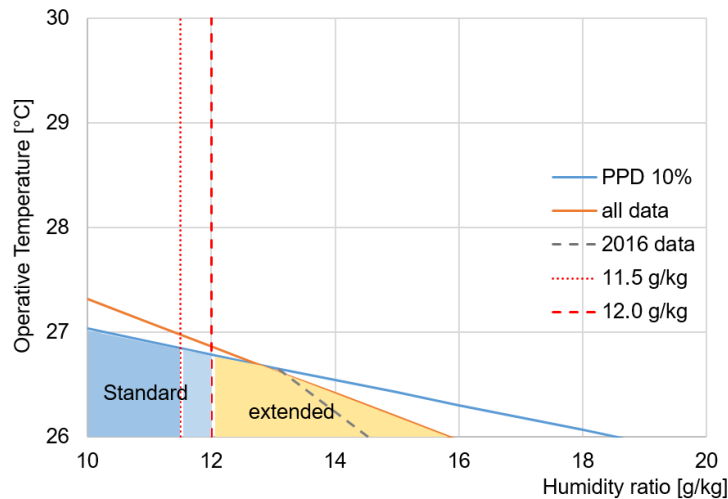
Figure 3. Extended comfort zone based on a HR/ t_o relation, derived from experiments with t_o > 26^\circ\text{C} and HR > 10 \text{ g/kg}
