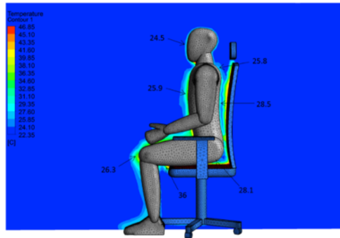
Figure 3. Temperature distribution around a manikin with the thermal chair. Shahzad (2017)
