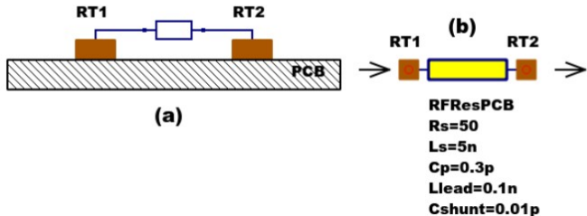
Verilog-A model
