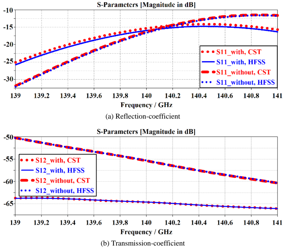
Fig. 2. Reflection ( S_{11} ) and transmission-coefficient ( S_{12} ) response of the proposed antenna array before and after implementing MSWI.
