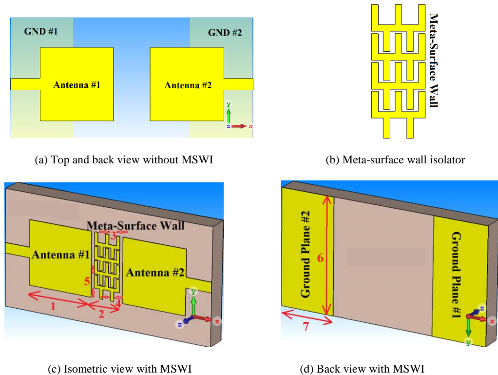
Fig. 1. Layout of the antenna array with and without the proposed meta-surface wall isolator. Dimensions of the numerical labels in (c) and (d) are given in Table 1.
