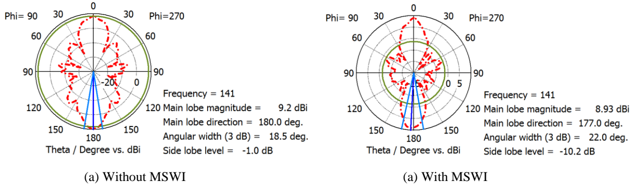
Fig. 4. Radiation patterns of the antenna array in the H-plane without and with MSWI at 139 GHz, 140 GHz, and 141 GHz.
