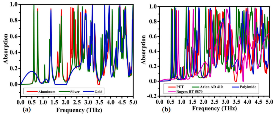
Fig. 4. Simulated absorption profiles showing (a) the influence of resonator materials and (b) variations due to substrate selection.
