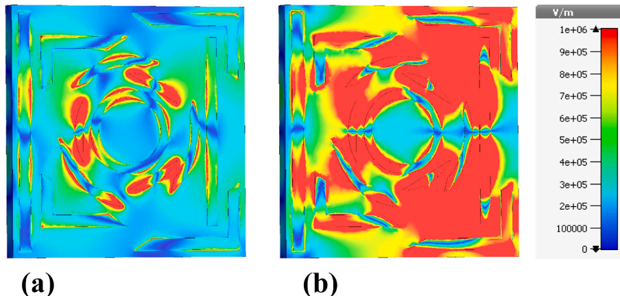
Fig. 9. Distribution of the electric field ( |E| ) across the resonator structure: (a) real field component, and (b) imaginary component.
