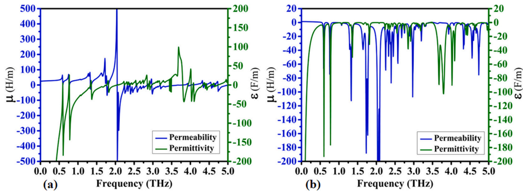
Fig. 7. Effective Electromagnetic Parameter Retrieval: (a) Real components of effective permittivity ( \epsilon ) and permeability ( \mu ), and (b) corresponding imaginary components.
