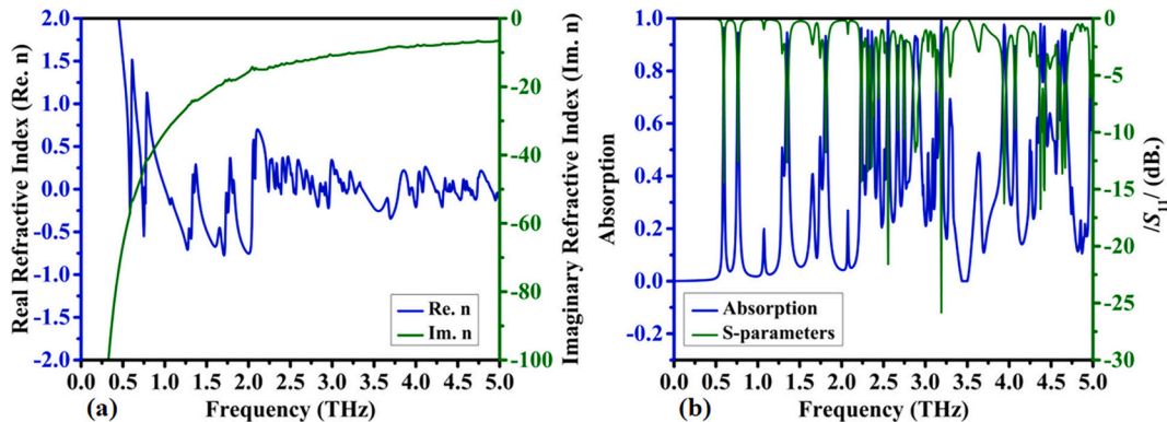
Fig. 8. Refractive Index and Reflection Analysis: (a) Real and imaginary components of the effective refractive index, and (b) reflection coefficient |S_{11}| in decibels (dB).
