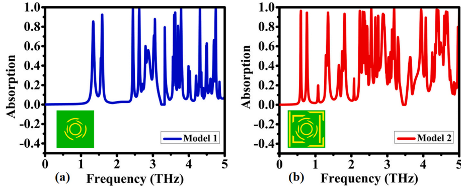
Fig. 3. Simulated absorption spectra of the proposed metamaterial absorber during the design evolution process: (a) Model 1 representing the initial resonator configuration and (b) Model 2 representing the optimized geometry. The comparison demonstrates the effect of the structural modifications on the resonance distribution, absorption characteristics, and multiband sensing performance of the proposed biosensor.
