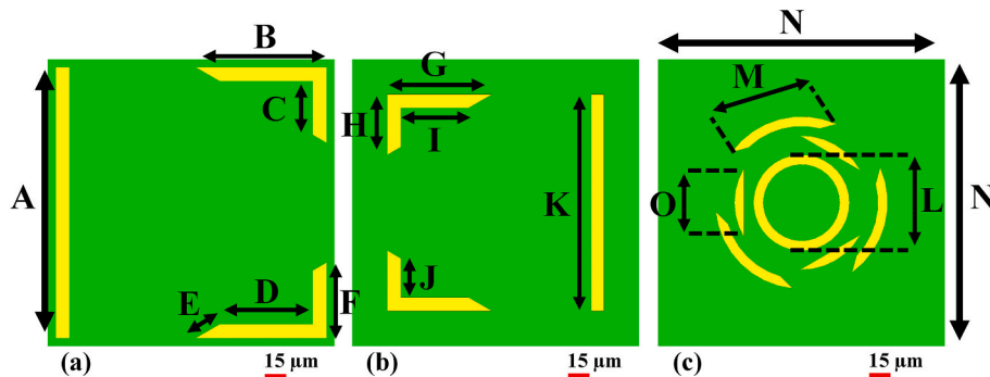
Fig. 1. Conceptual representation of the proposed metamaterial absorber integrating three design stages: (a) Initial prototype (Design Variant 1), (b) Intermediate configuration (Design Variant 2), and (c) Final optimized sensor architecture (Design Variant 3).
