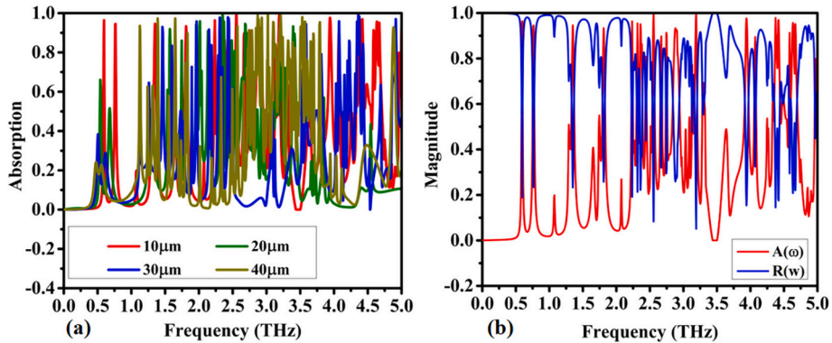
Fig. 5. Performance results demonstrating (a) the effect of substrate thickness on absorption magnitude and (b) comparative reflection and absorption characteristics across the operating frequency spectrum.
