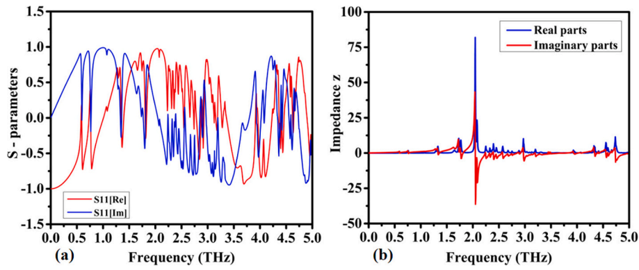
Fig. 6. S-Parameter and Impedance Characterization: (a) Real and imaginary components of the reflection coefficient ( S_{11} ), and (b) normalized impedance variation across the frequency spectrum.
