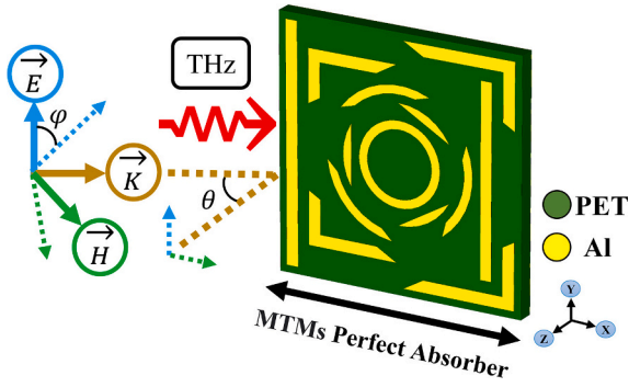
Fig. 2. Schematic depiction of the absorber arrangement showing the orientation of the incident terahertz wave relative to the stratified layer geometry.
