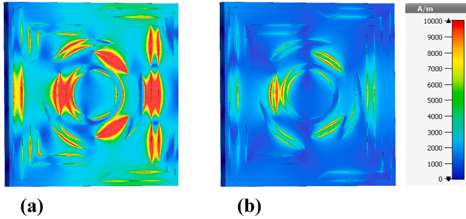
Fig. 10. Visualization of magnetic field ( |H| ) distribution within the metamaterial design: (a) real part, (b) imaginary part.
