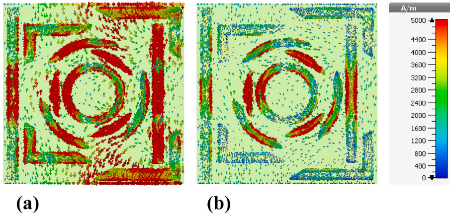
Fig. 11. Simulated surface current flow over the resonator structure: (a) real component, (b) imaginary component.
