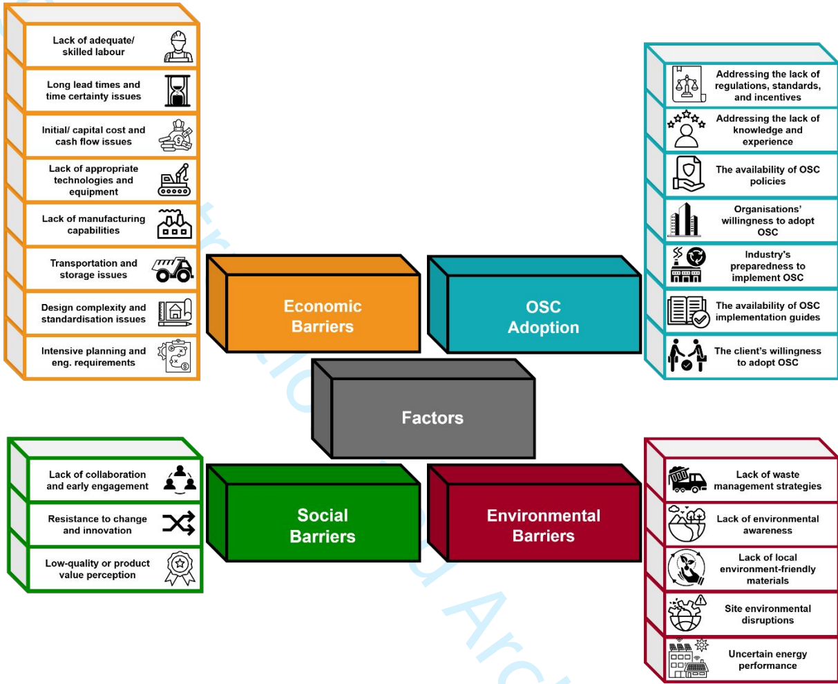
Figure 1: Results of Factor Analysis
