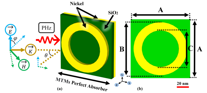
Fig. 1. Structural design and incident field orientations of a recommended perfect absorber; (a) schematic representation of the structural design and incident field orientations of a perfect absorber, and (b) proposed design model.
