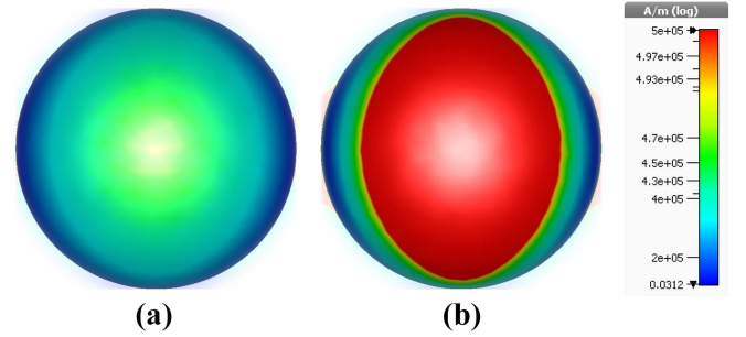
Fig. 17. MWI visualization of the magnetic field (H-field) at 400 THz, examining exosomes with the near-infrared biosensor: (a) Normal exosomes, and (b) cancerous exosomes.
