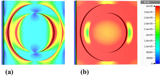
Fig. 11. Visualization of metamaterial structure field distributions on a color map: (a) Real parts of |H| -field, and (b) imaginary parts of |H| -field.
