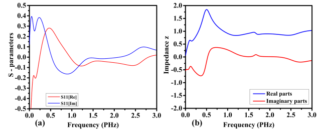
Fig. 5. The simulated responses of parameters of the proposed model: (a) S_{11} real and imaginary parts, and (b) impedance z .
