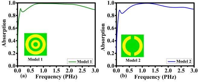
Fig. 2. Comparison of absorption properties between two distinct designs: (a) Absorption properties of model 1, and (b) absorption properties of model 2.
