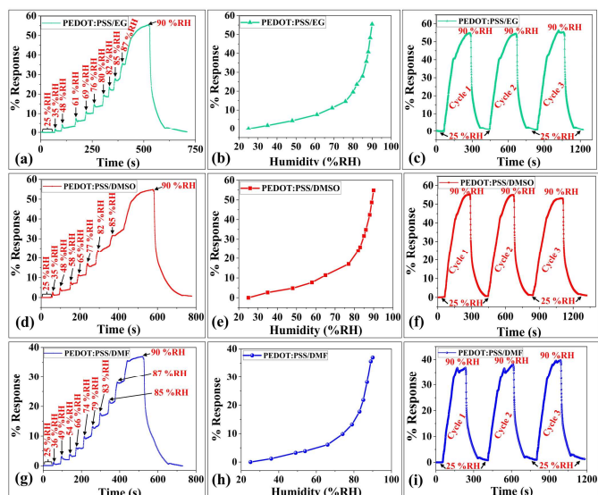
Fig. 4. Humidity sensing characteristics in range 25-90%RH of the (a-c) PEDOT:PSS/EG sensor: (a) dynamic humidity sensing characteristics (b) % response vs humidity graph (c) 3-cyclic repeatability analysis; (d-f) PEDOT:PSS/DMSO sensor: (d) dynamic humidity sensing characteristics (e) % response vs humidity graph (f) 3-cyclic repeatability analysis; (g-i) PEDOT:PSS/DMF sensor: (g) dynamic humidity sensing characteristics (h) % response vs humidity graph (i) 3-cyclic repeatability analysis.
