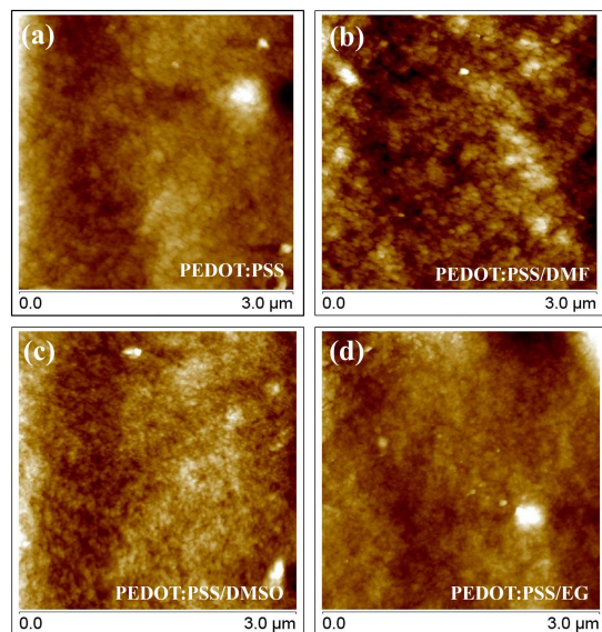
Fig. 3. AFM images of the (a) pristine PEDOT:PSS (b) PEDOT:PSS/DMF (c) PEDOT:PSS/DMSO and (d) PEDOT:PSS/EG at 3 μm scales.
