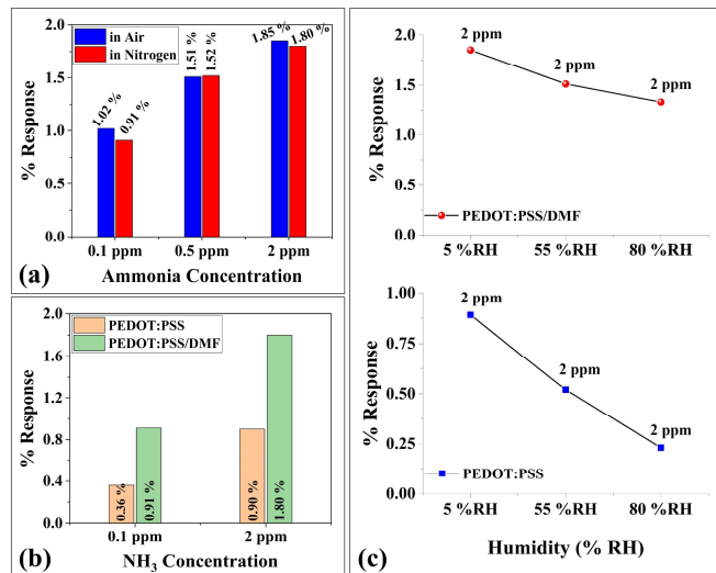
Fig. 8. Understanding the impact of DMF additive on ammonia gas sensing performance of PEDOT:PSS at room temperature in N 2 and air environment. (a) % Response vs concentration graph for PEDOT:PSS/DMF sensor at 0.1 ppm, 0.5 ppm and 2 ppm of ammonia in air and N 2 environment. (b) Comparative analysis on the sensing performance of pristine PEDOT:PSS and PEDOT:PSS/DMF sensors at 0.1 ppm and 2 ppm of ammonia. (c) Effect of relative humidity on ammonia gas sensing properties of PEDOT:PSS/DMF sensor as compared to pristine PEDOT:PSS at 2 ppm of ammonia concentration.
