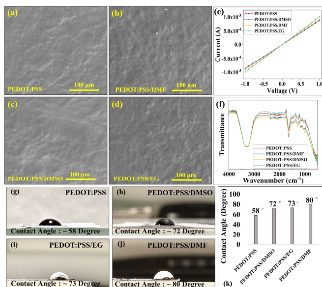
Fig. 2. SEM images of the (a) pristine PEDOT:PSS (b) PEDOT:PSS/DMF (c) PEDOT:PSS/DMSO and (d) PEDOT:PSS/EG at 100 \mu m scales. (e) I-V characteristics comparison and analysis. (f) FTIR analysis. Contact angle measurements for (g) pristine PEDOT:PSS; (h) PEDOT:PSS/DMSO; (i) PEDOT:PSS/EG; (j) PEDOT:PSS/DMF. (k) Comparative analysis of the obtained contact angles.
