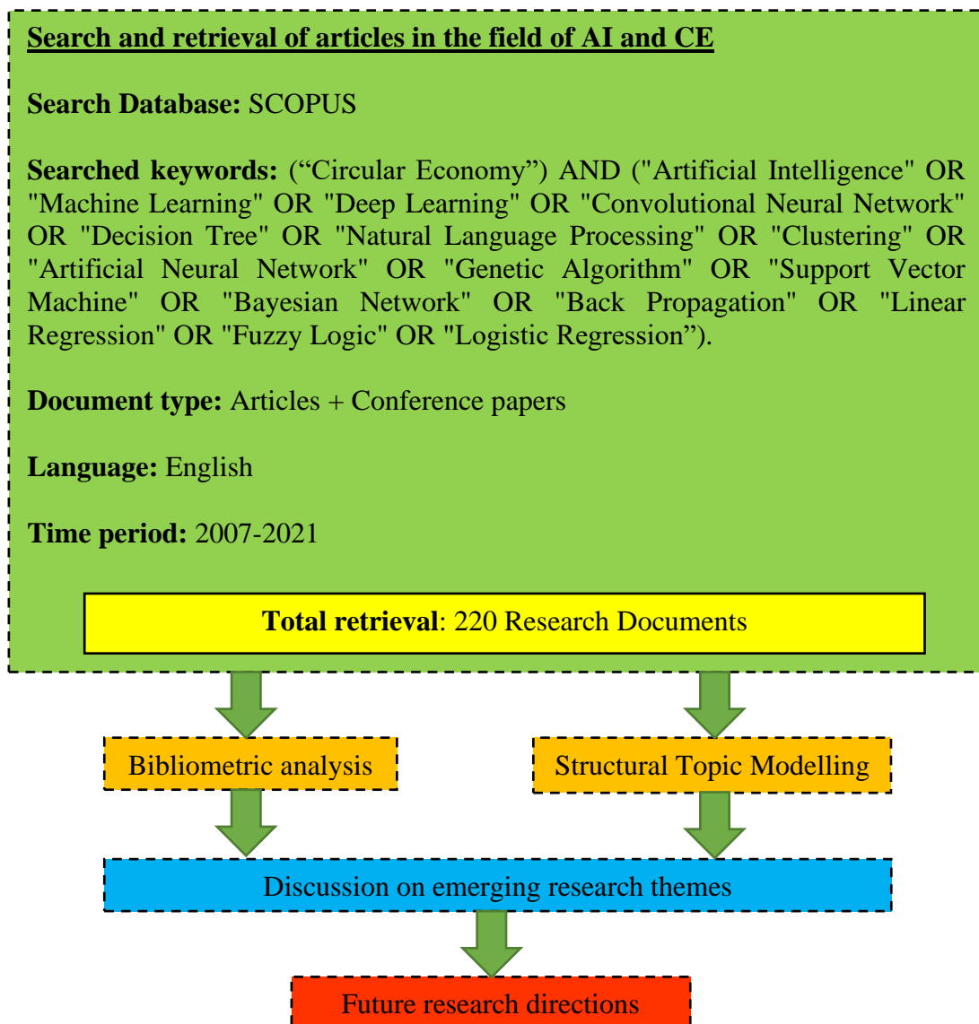
Figure 1. SLR flowchart
